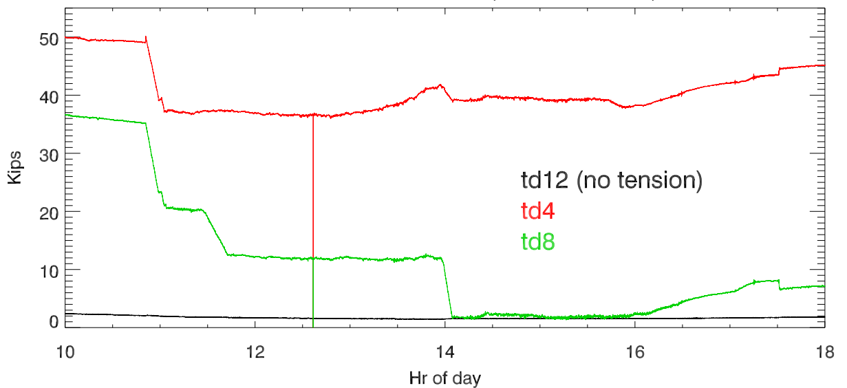
Tension in each td corner (sum of 2 cables)
