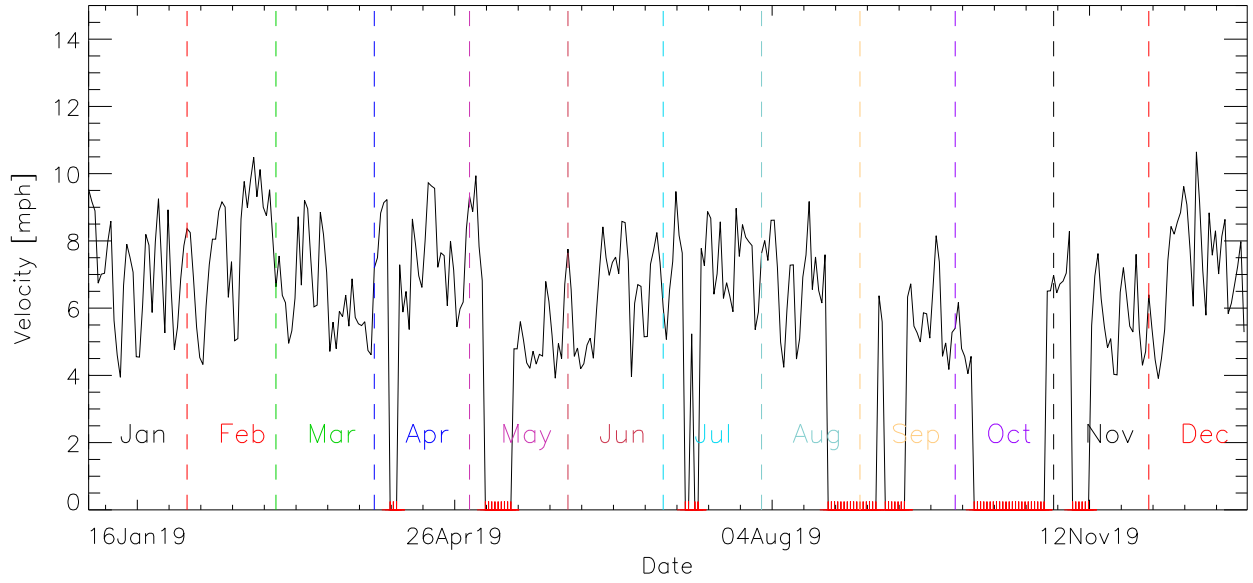
2019 Maximum daily velocity
