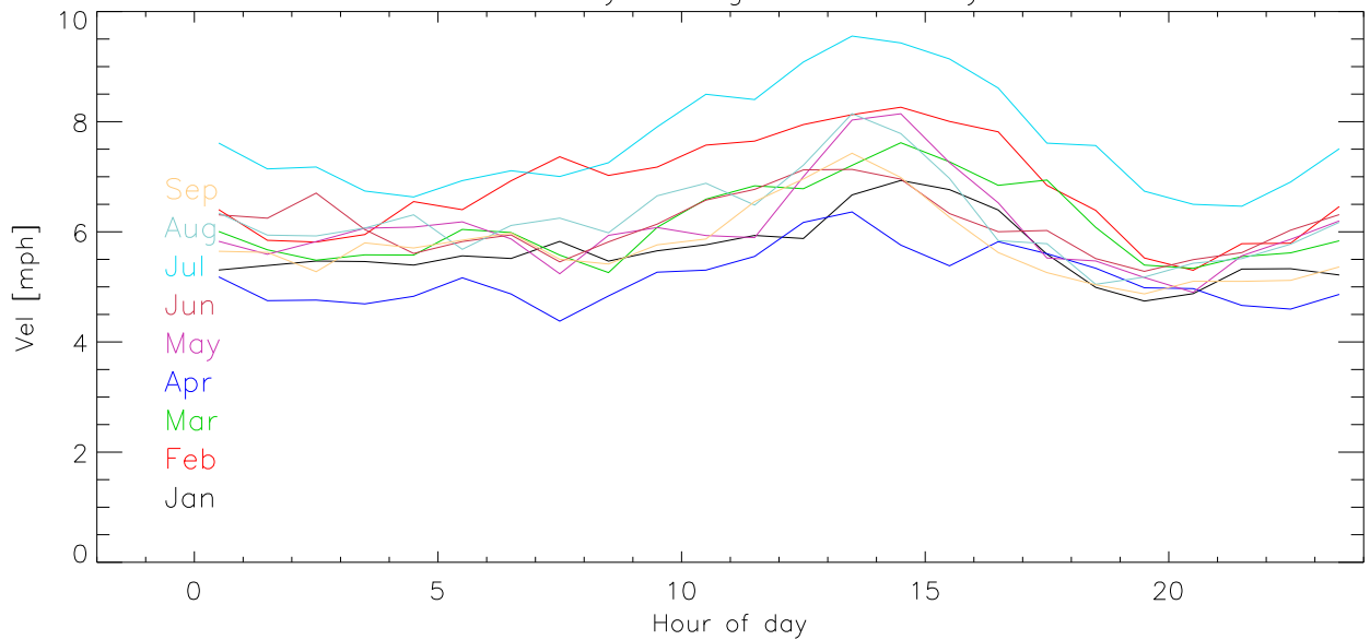
2003 Monthly average wind velocity vs hour
