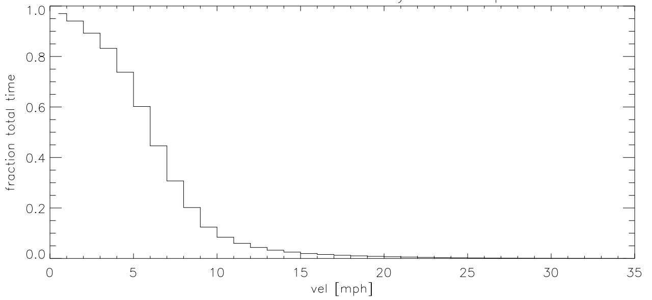
AUG20 Fraction of time wind velocity exceeds specified vel (blowup)
