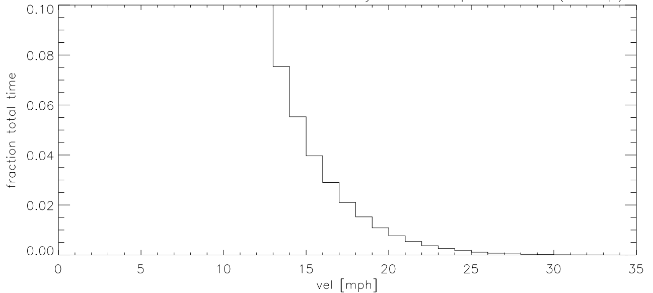
MAR20 Fraction of time wind velocity exceeds specified vel (blowup)
