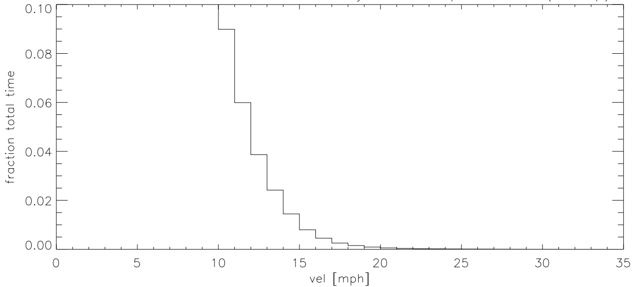
JUN19 Fraction of time wind velocity exceeds specified vel (blowup)
