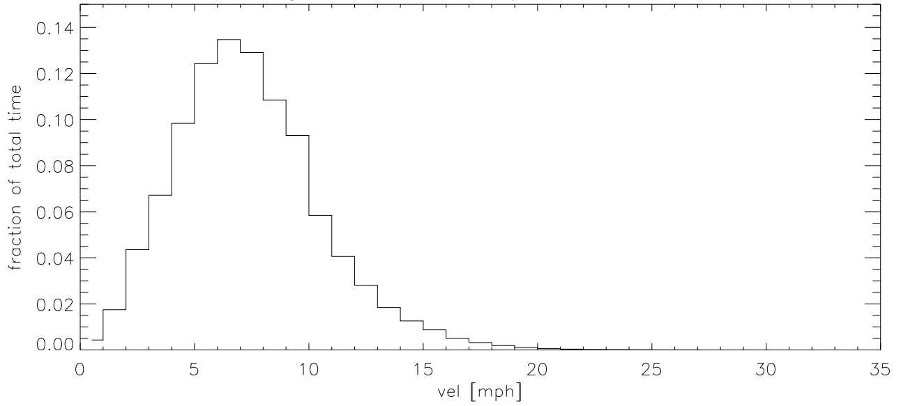
AUG18 Fraction of time wind velocity exceeds specified vel
