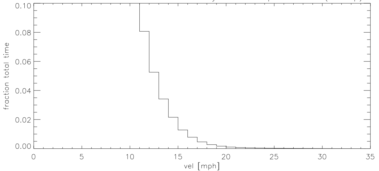
AUG18 Fraction of time wind velocity exceeds specified vel (blowup)
