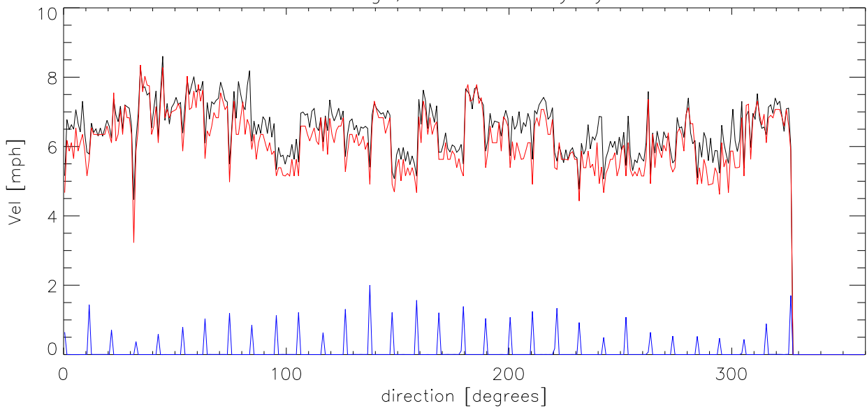
NOV17 Average, median velocity by direction
