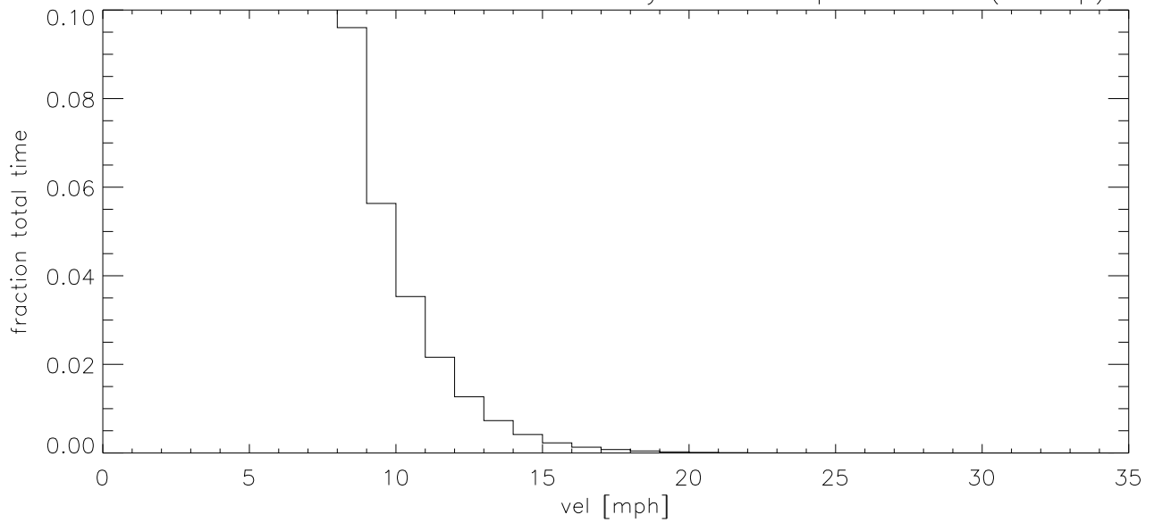
NOV17 Fraction of time wind velocity exceeds specified vel (blowup)
