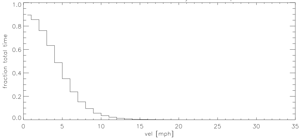
NOV17 Fraction of time wind velocity exceeds specified vel (blowup)
