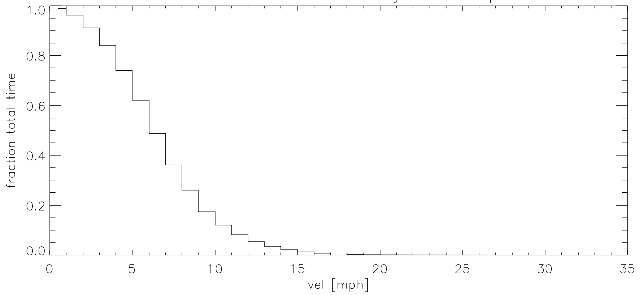
AUG17 Fraction of time wind velocity exceeds specified vel (blowup)
