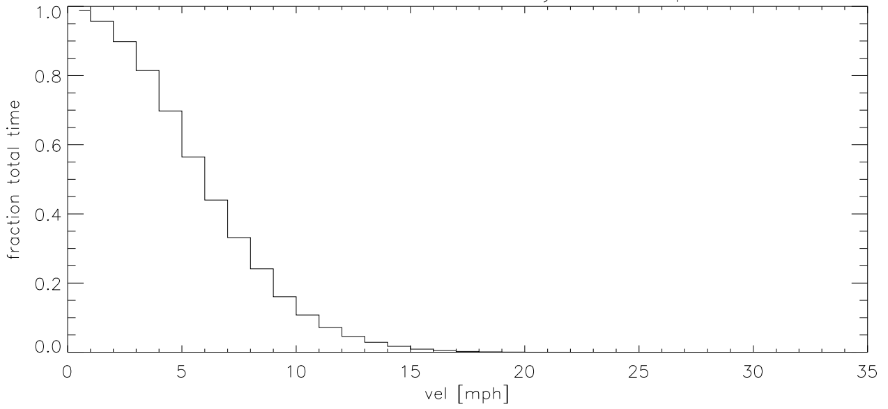
JUN17 Fraction of time wind velocity exceeds specified vel (blowup)
