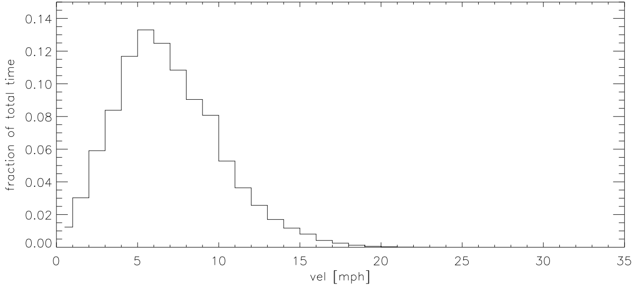
JUN17 Fraction of time wind velocity exceeds specified vel
