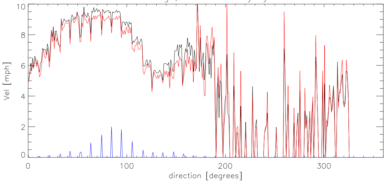
DEC15 Average, median velocity by direction
