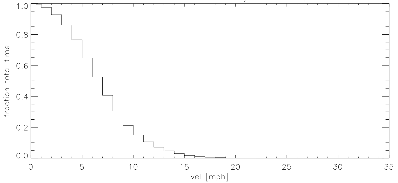
DEC15 Fraction of time wind velocity exceeds specified vel (blowup)
