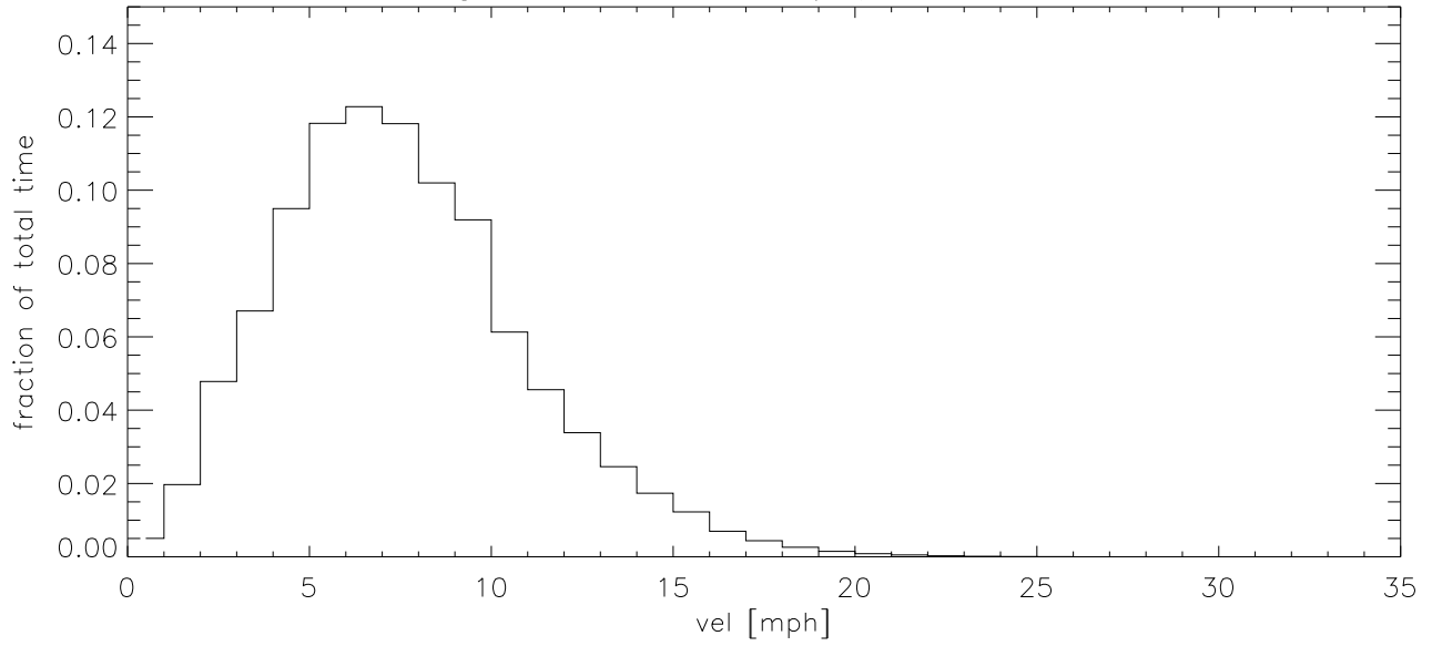
DEC15 Fraction of time wind velocity exceeds specified vel
