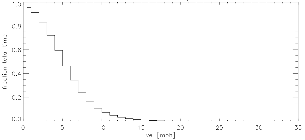
JUN15 Fraction of time wind velocity exceeds specified vel (blowup)
