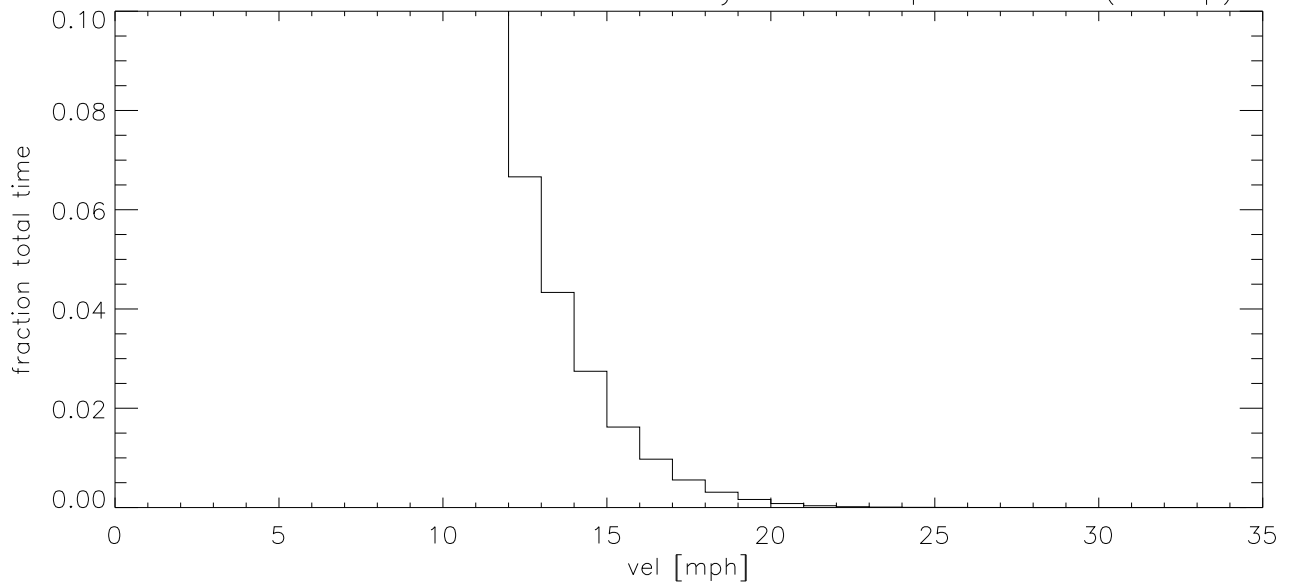
JAN14 Fraction of time wind velocity exceeds specified vel (blowup)
