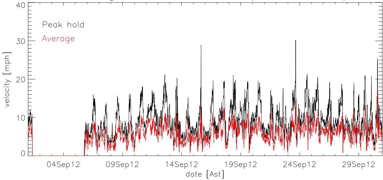
SEP12 Average, median velocity by hour of day
