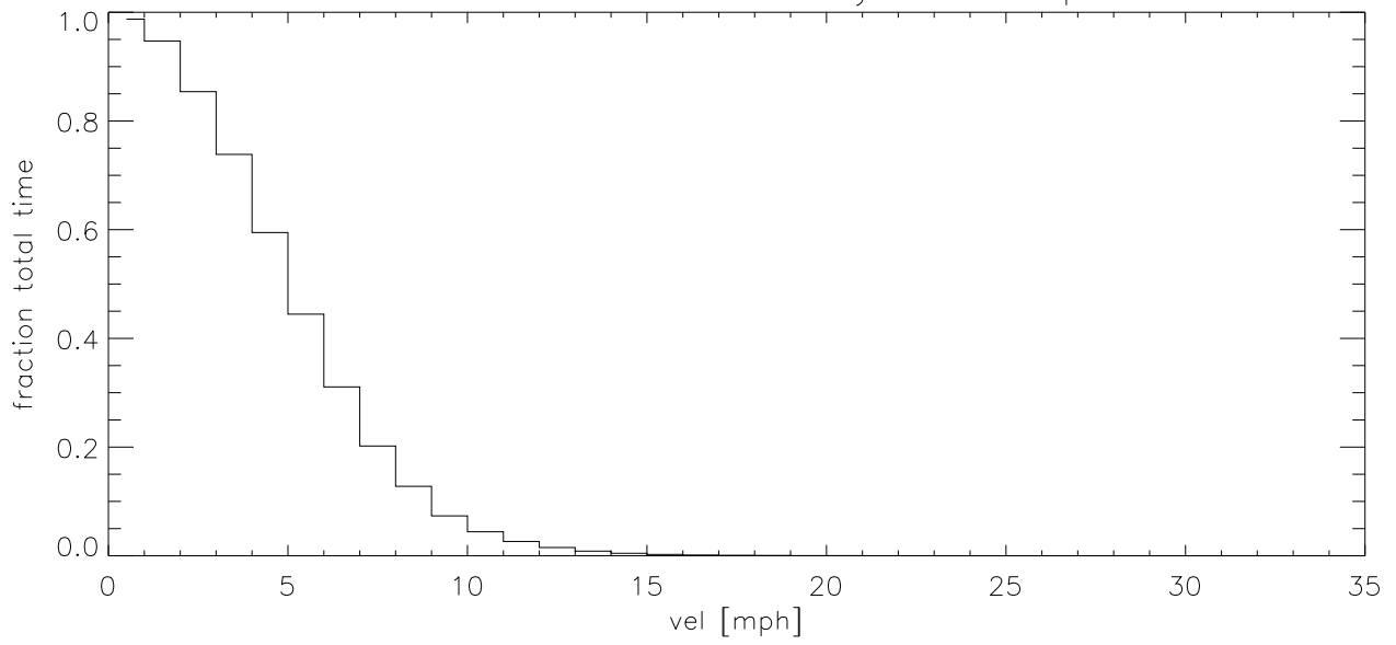
SEP12 Fraction of time wind velocity exceeds specified vel (blowup)
