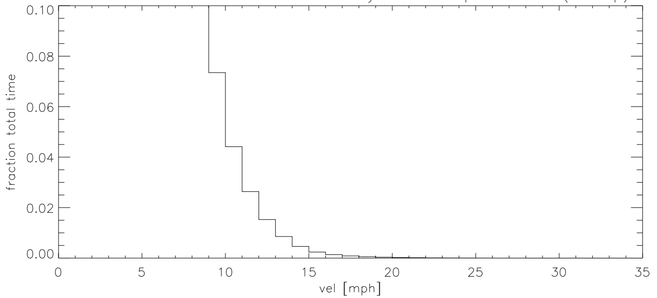
SEP12 Fraction of time wind velocity exceeds specified vel (blowup)
