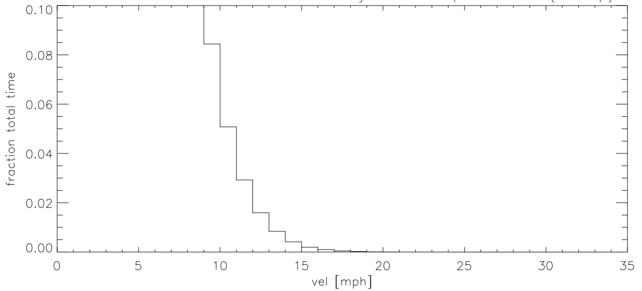
OCT11 Fraction of time wind velocity exceeds specified vel (blowup)
