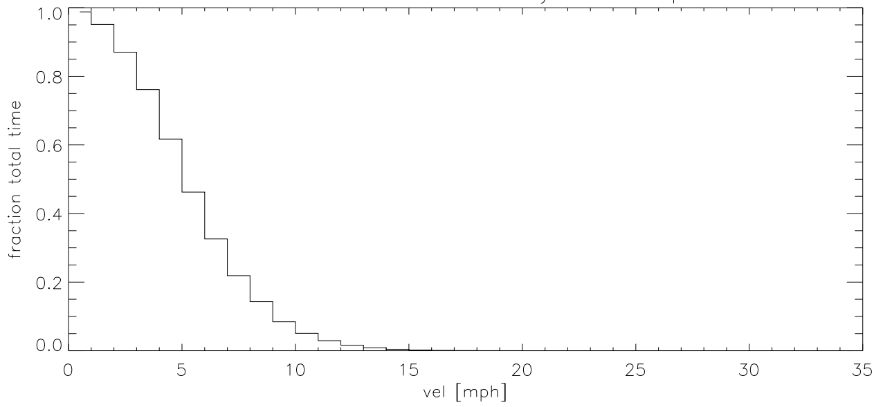
OCT11 Fraction of time wind velocity exceeds specified vel (blowup)
