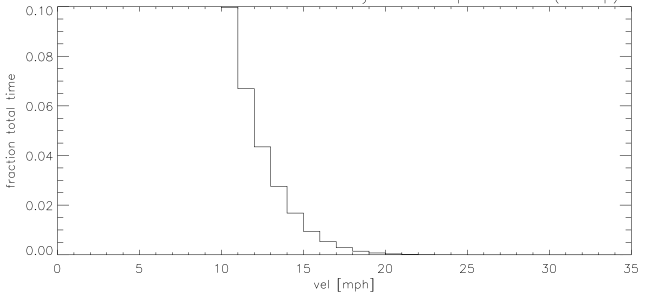
MAR11 Fraction of time wind velocity exceeds specified vel (blowup)
