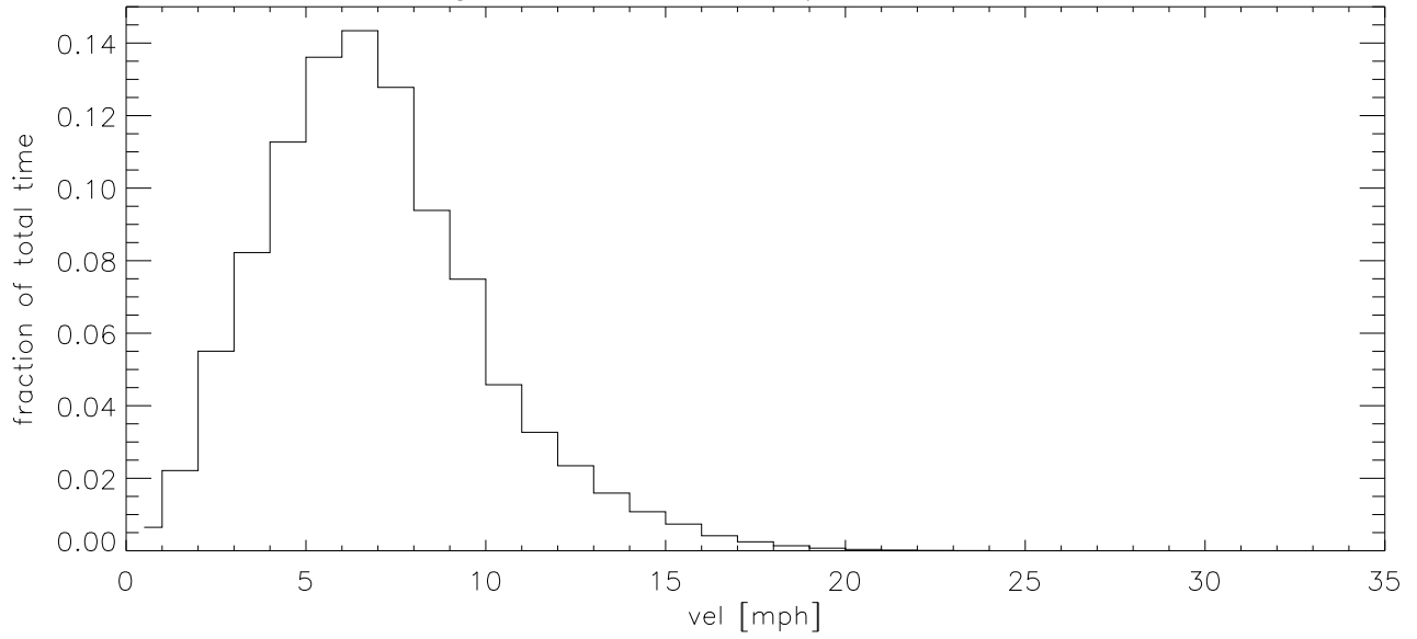
MAR11 Fraction of time wind velocity exceeds specified vel
