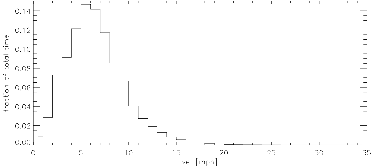
SEP10 Fraction of time wind velocity exceeds specified vel
