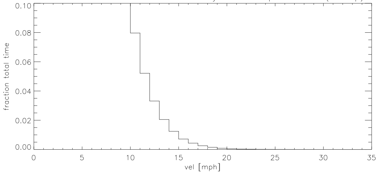
SEP10 Fraction of time wind velocity exceeds specified vel (blowup)
