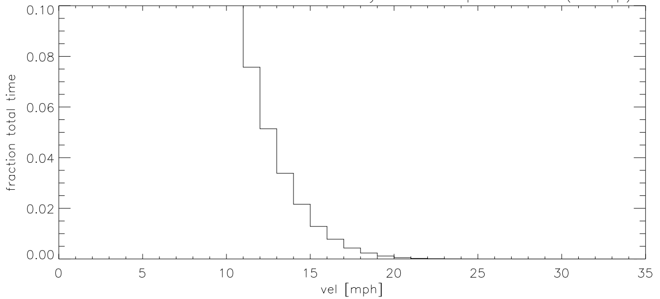
APR10 Fraction of time wind velocity exceeds specified vel (blowup)
