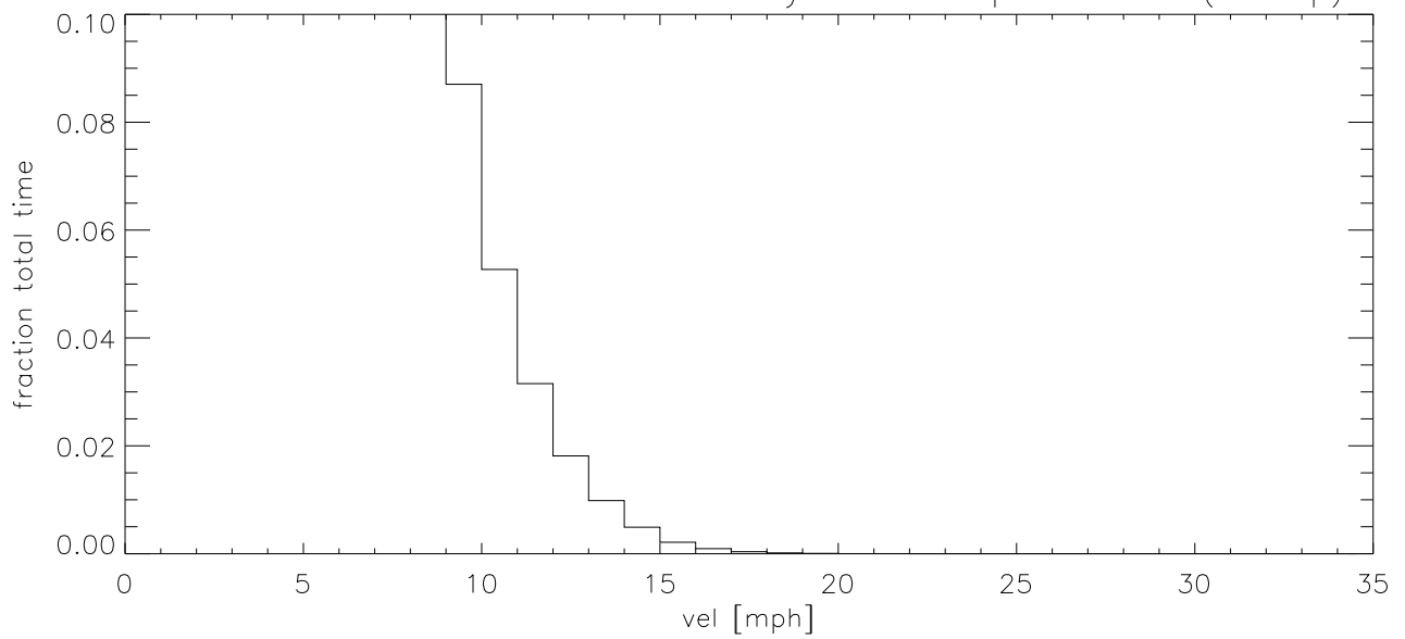
OCT09 Fraction of time wind velocity exceeds specified vel (blowup)
