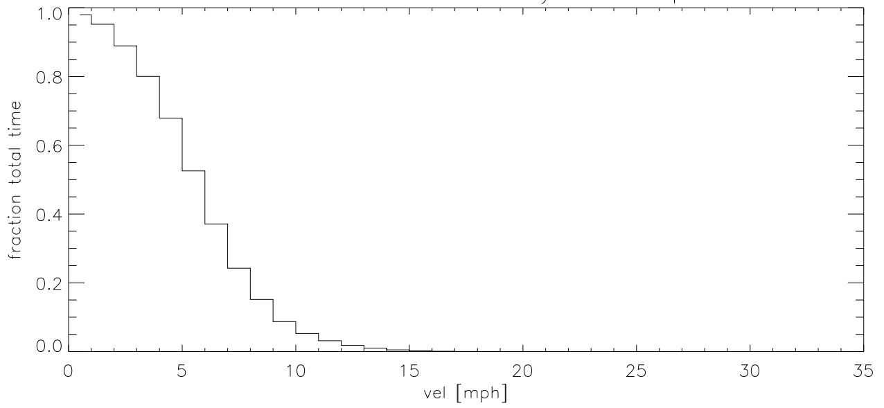
OCT09 Fraction of time wind velocity exceeds specified vel (blowup)
