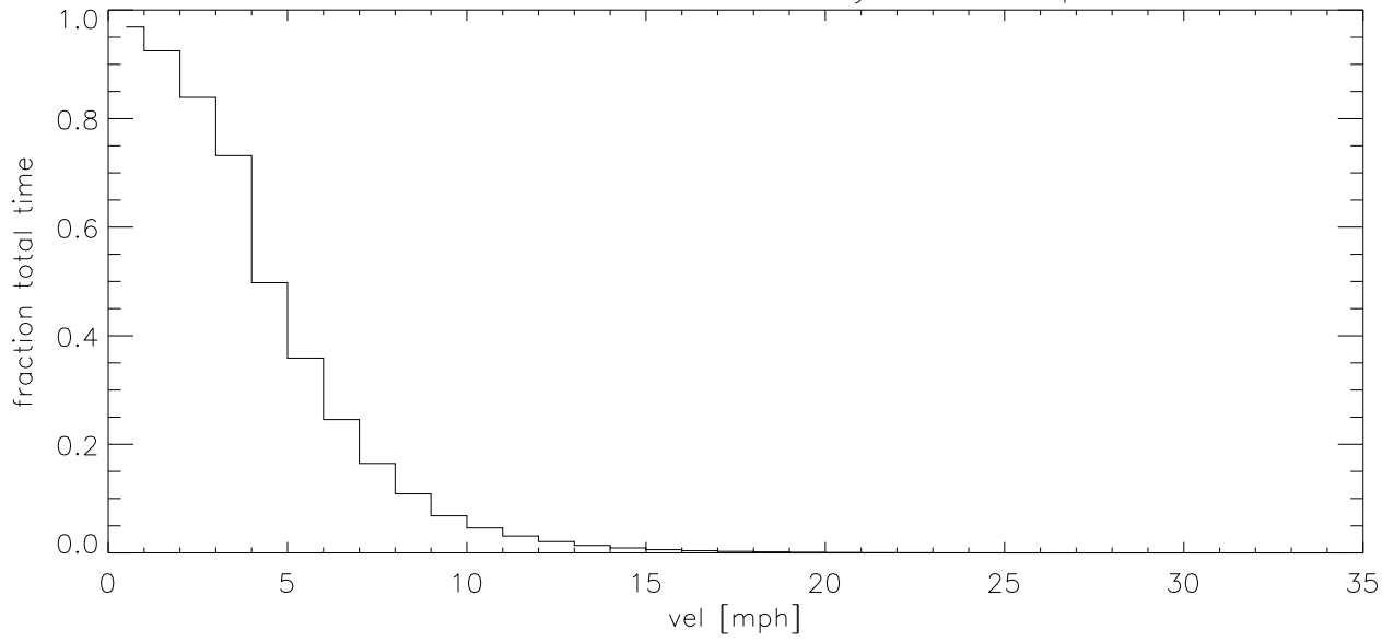
SEP09 Fraction of time wind velocity exceeds specified vel (blowup)
