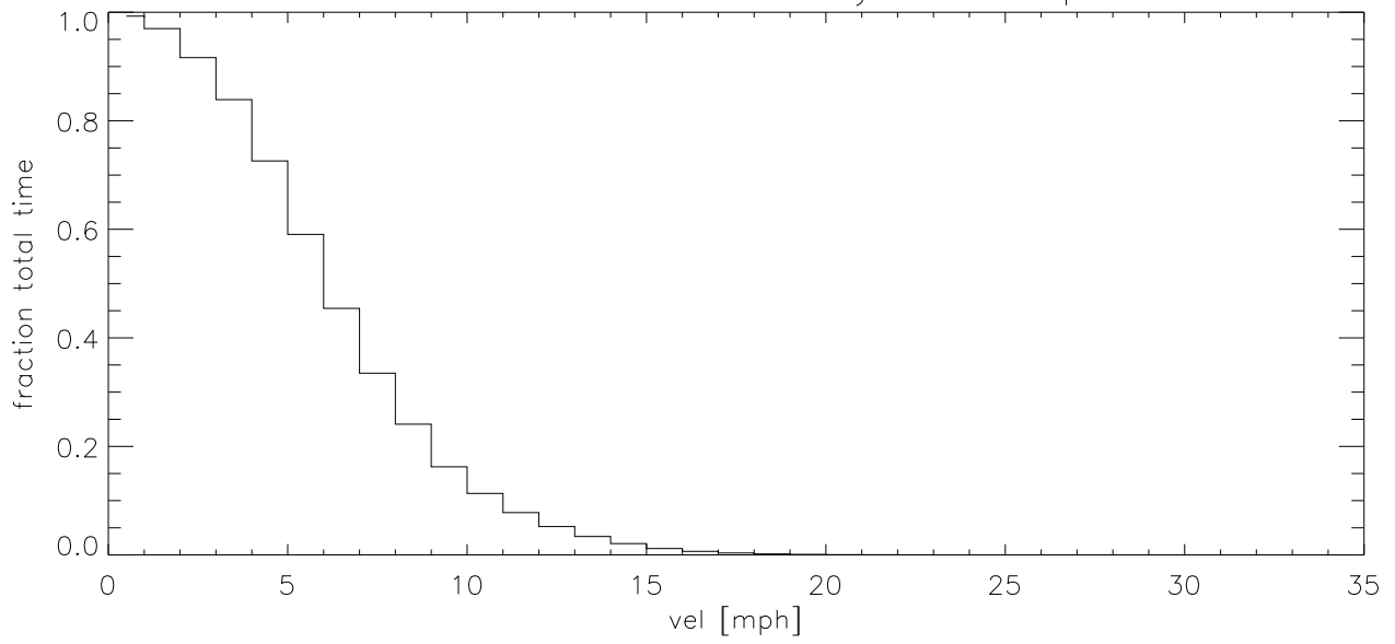
AUG09 Fraction of time wind velocity exceeds specified vel (blowup)
