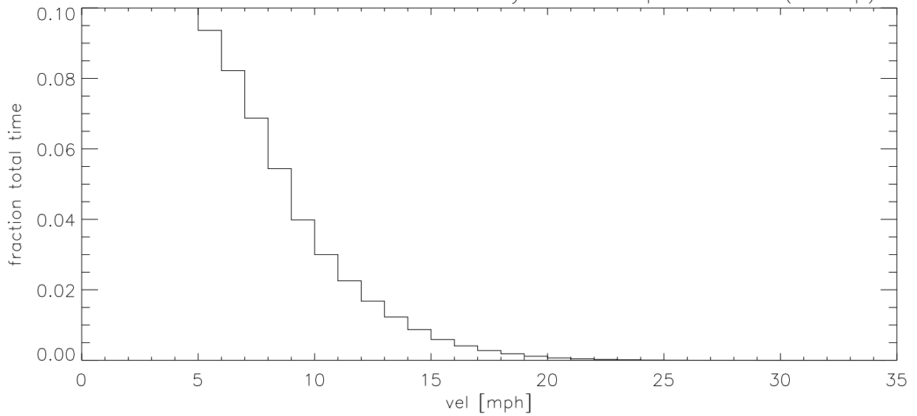
JUL09 Fraction of time wind velocity exceeds specified vel (blowup)
