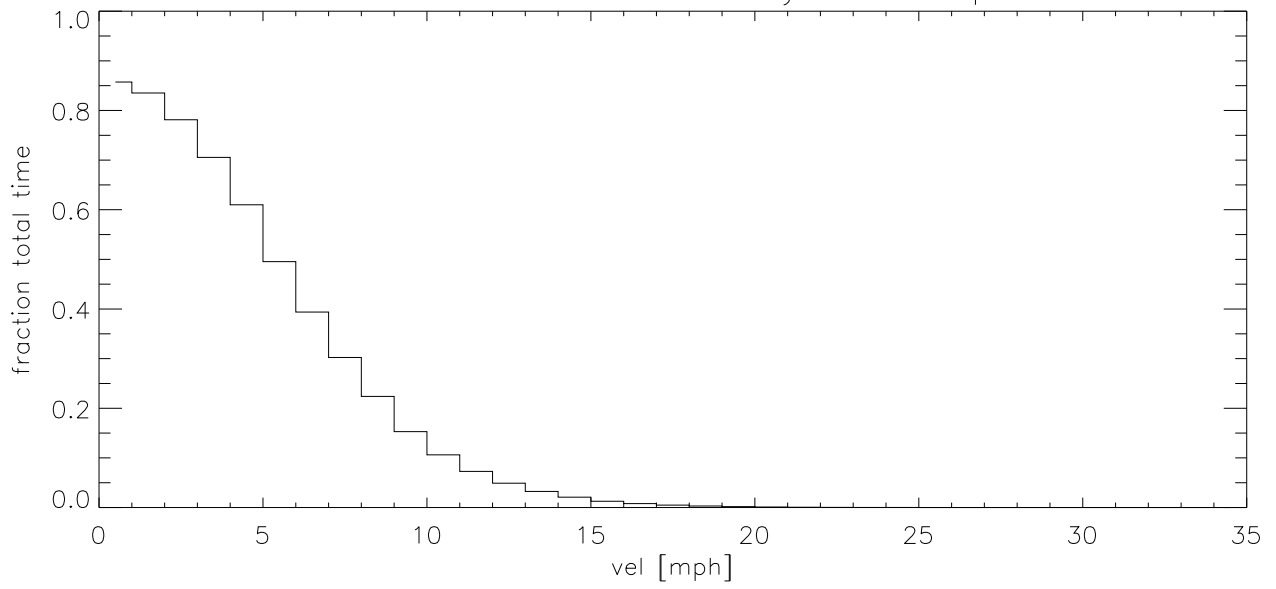
MAR09 Fraction of time wind velocity exceeds specified vel (blowup)
