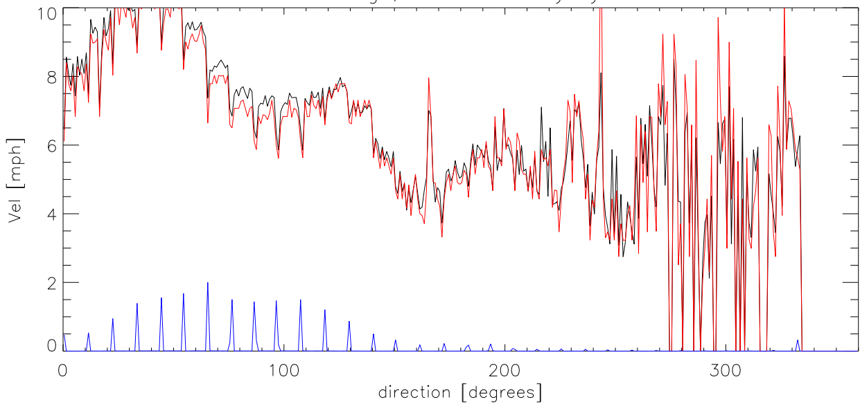
MAR09 Average, median velocity by direction
