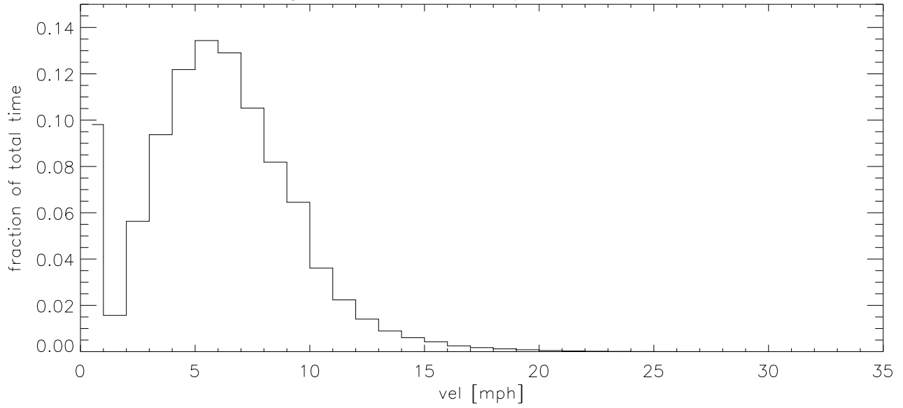
NOV08 Fraction of time wind velocity exceeds specified vel
