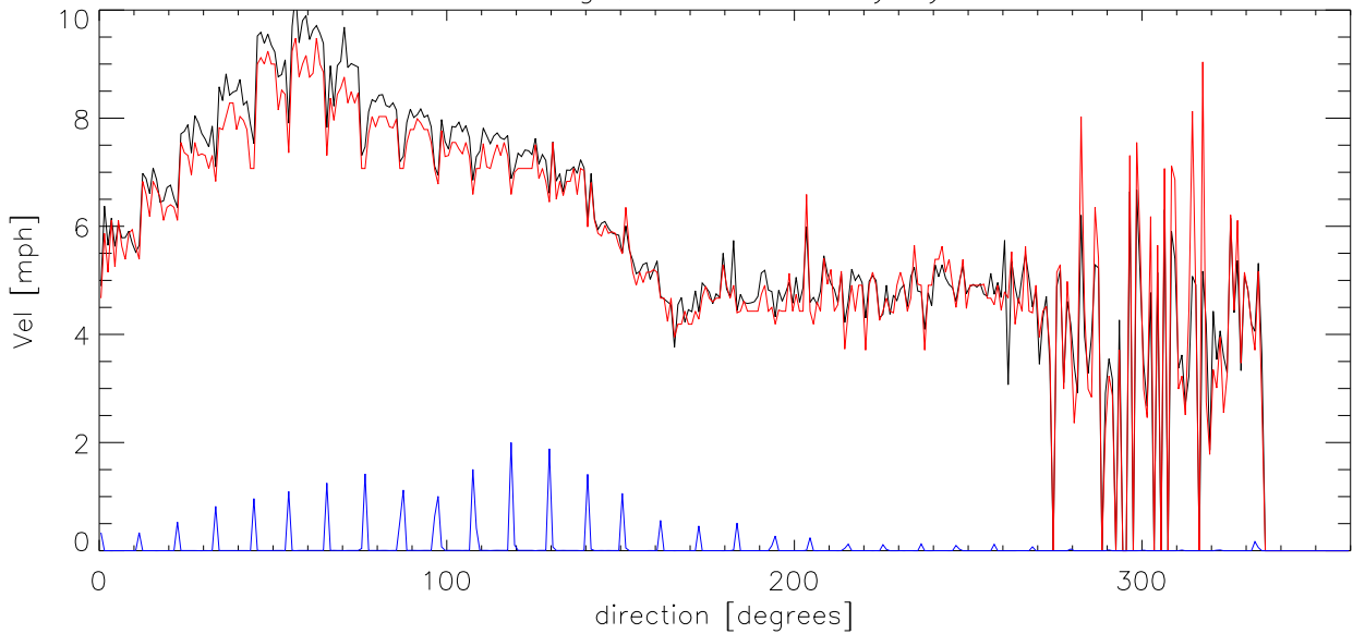
NOV08 Average, median velocity by direction
