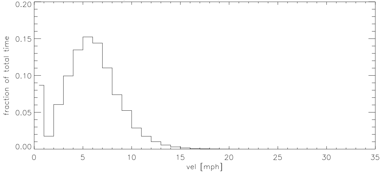
OCT08 Fraction of time wind velocity exceeds specified vel
