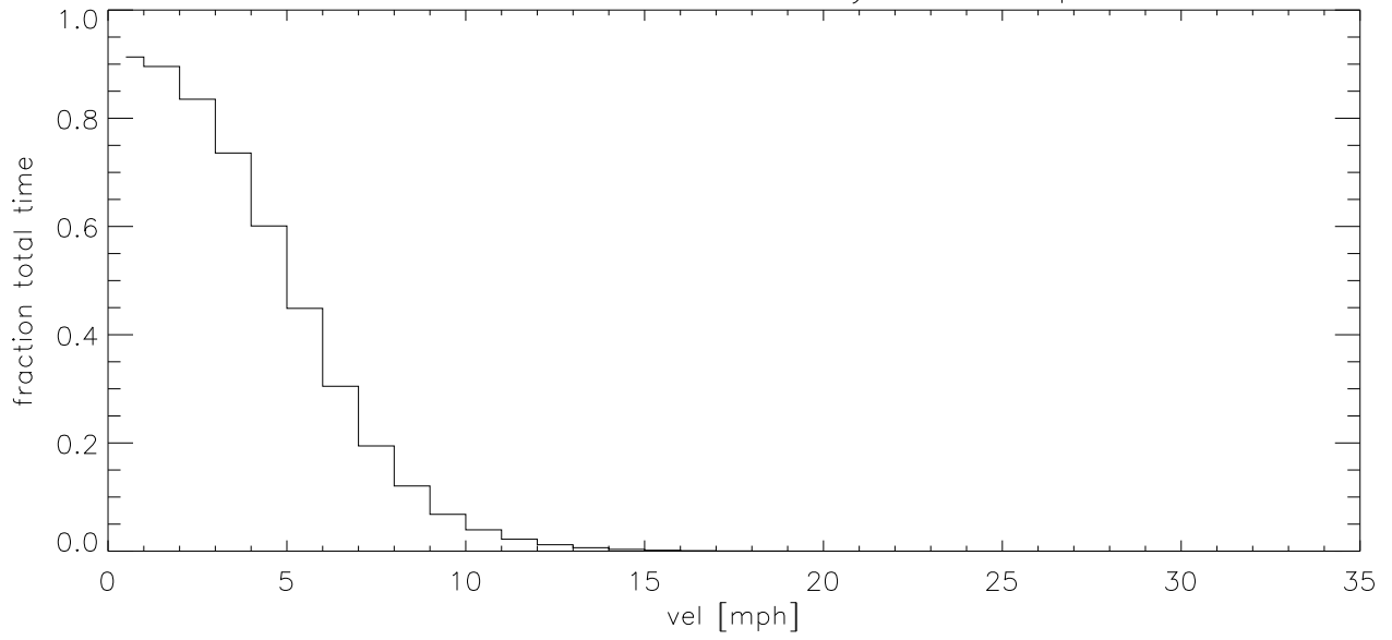
OCT08 Fraction of time wind velocity exceeds specified vel (blowup)
