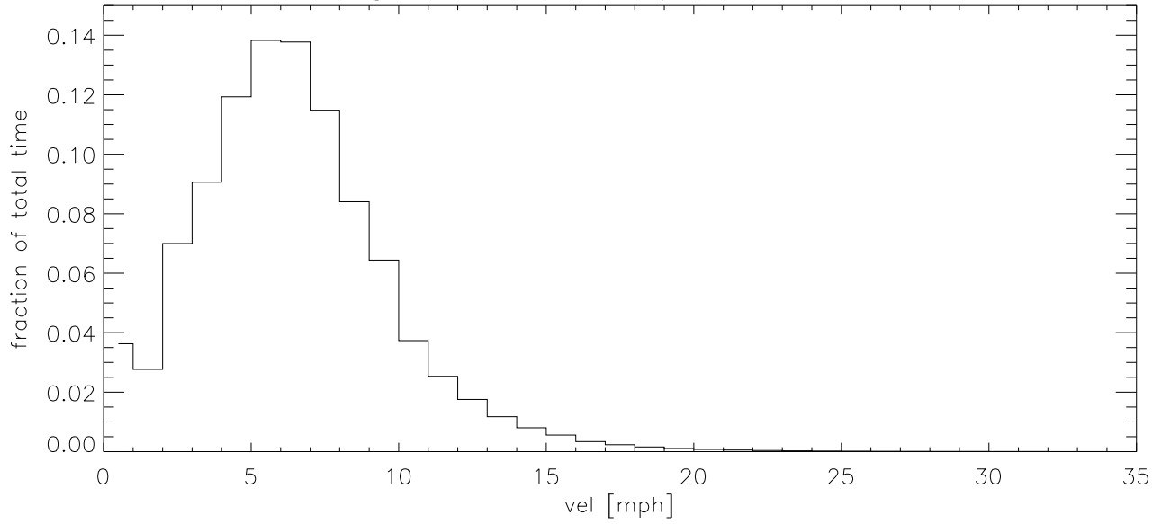
AUG08 Fraction of time wind velocity exceeds specified vel
