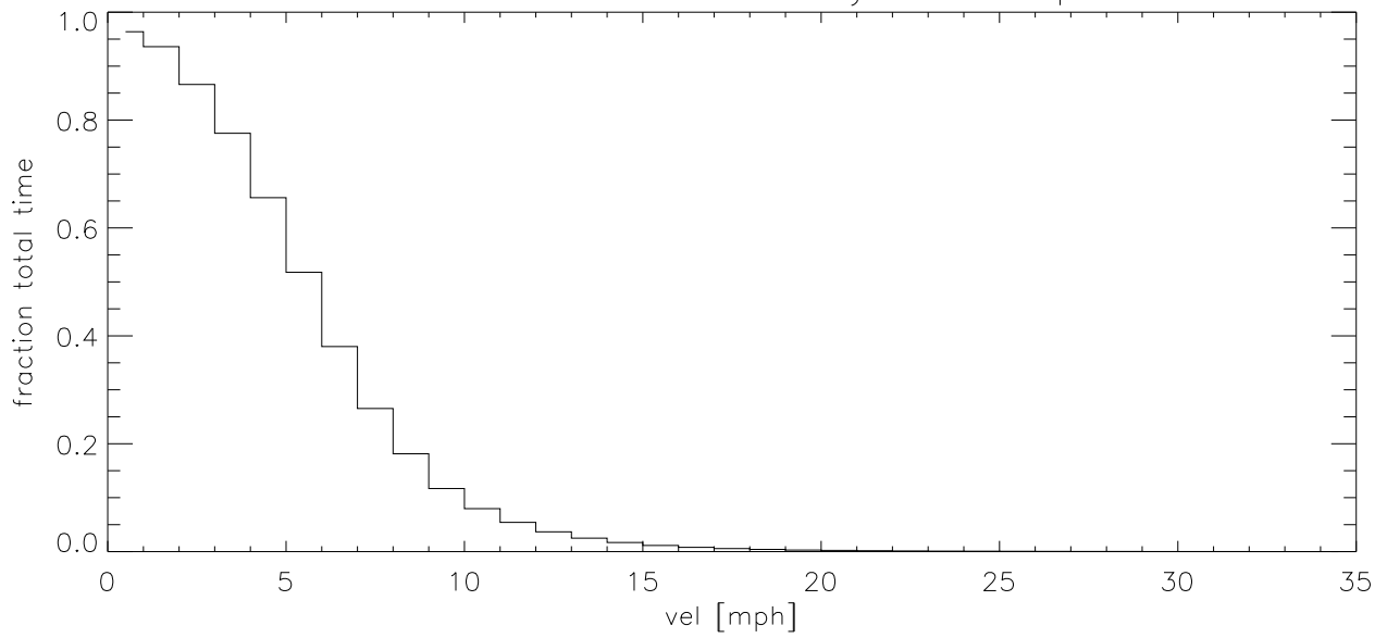
AUG08 Fraction of time wind velocity exceeds specified vel (blowup)
