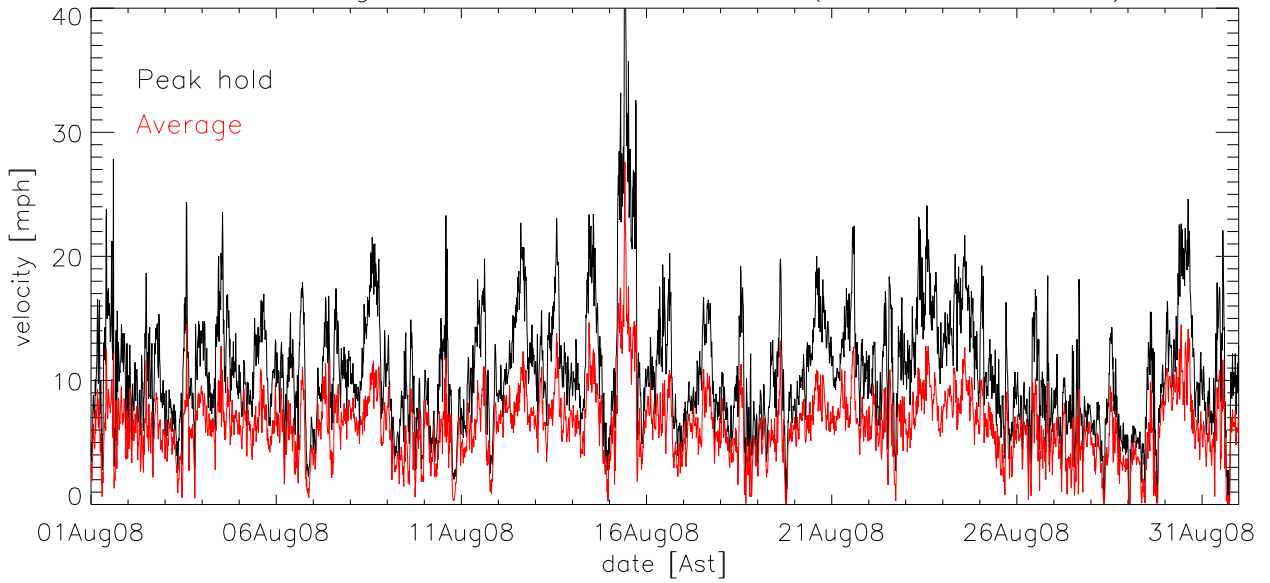
AUG08 Average, median velocity by hour of day
