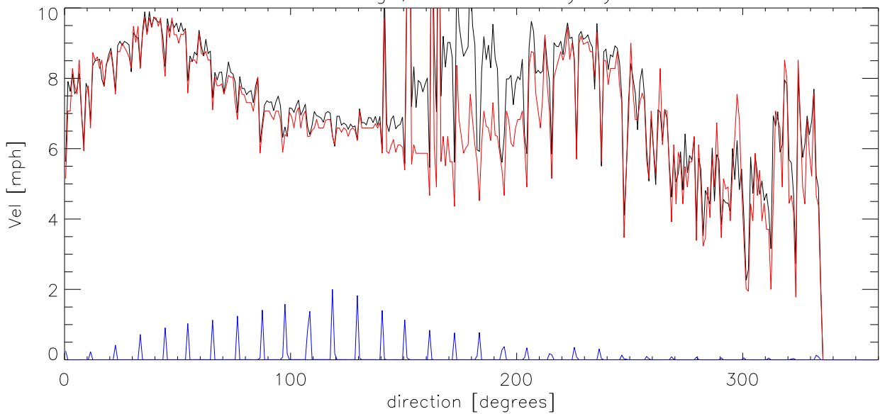
AUG08 Average, median velocity by direction
