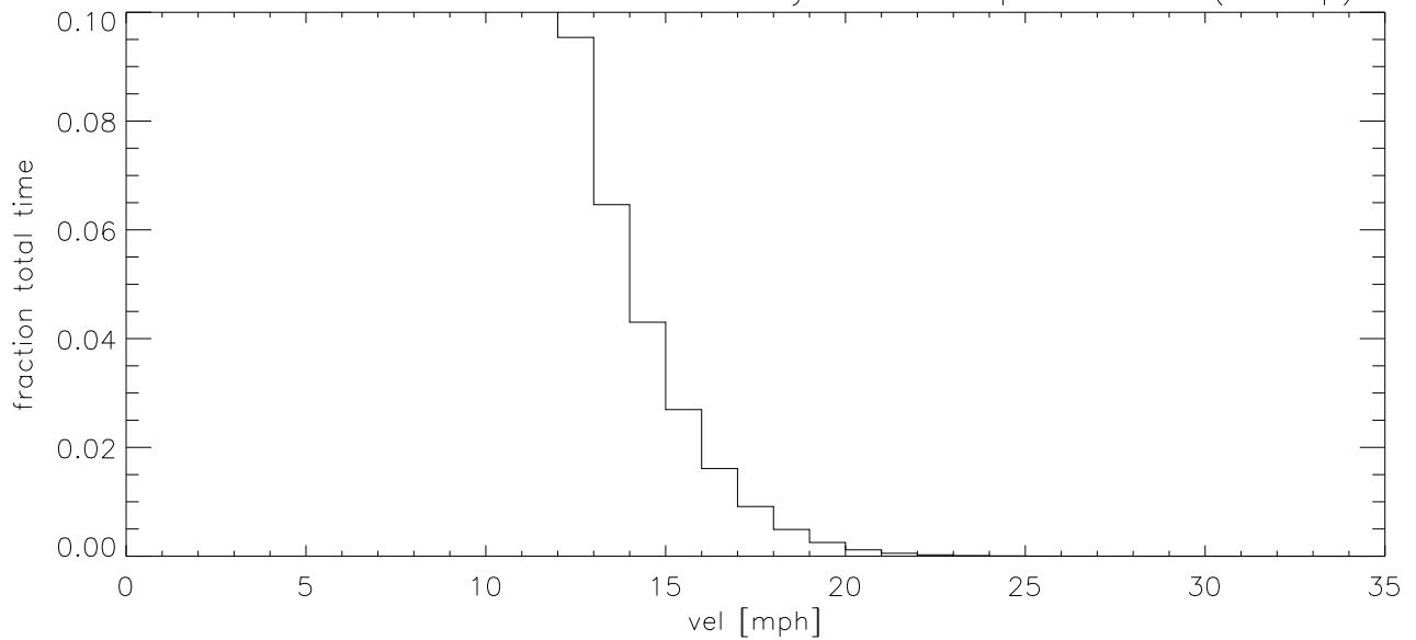
FEB08 Fraction of time wind velocity exceeds specified vel (blowup)
