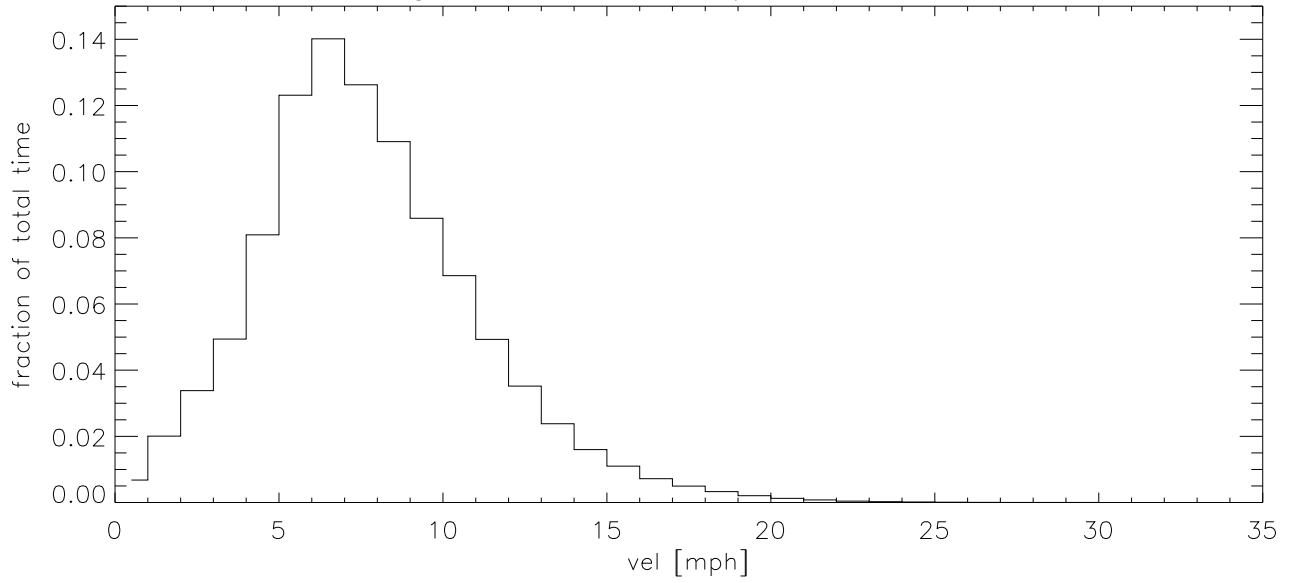
DEC07 Fraction of time wind velocity exceeds specified vel
