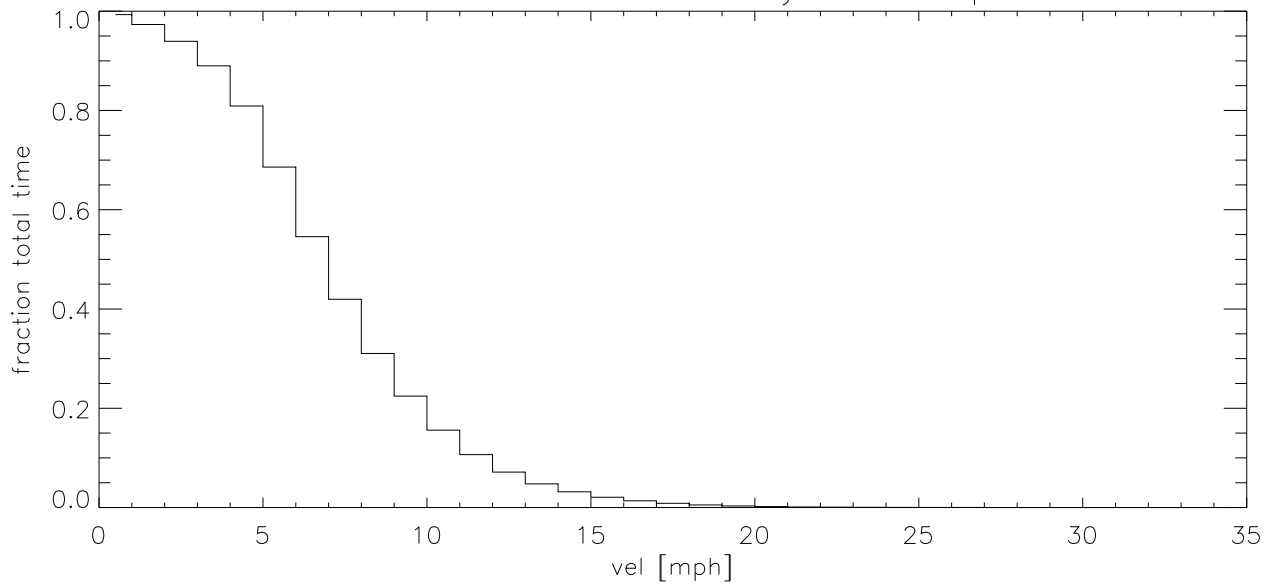
DEC07 Fraction of time wind velocity exceeds specified vel (blowup)
