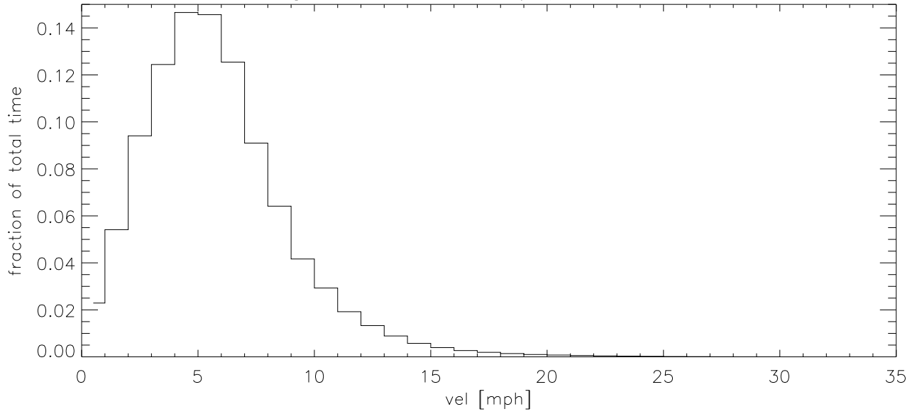
OCT07 Fraction of time wind velocity exceeds specified vel
