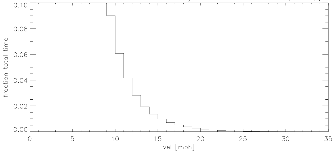
OCT07 Fraction of time wind velocity exceeds specified vel (blowup)
