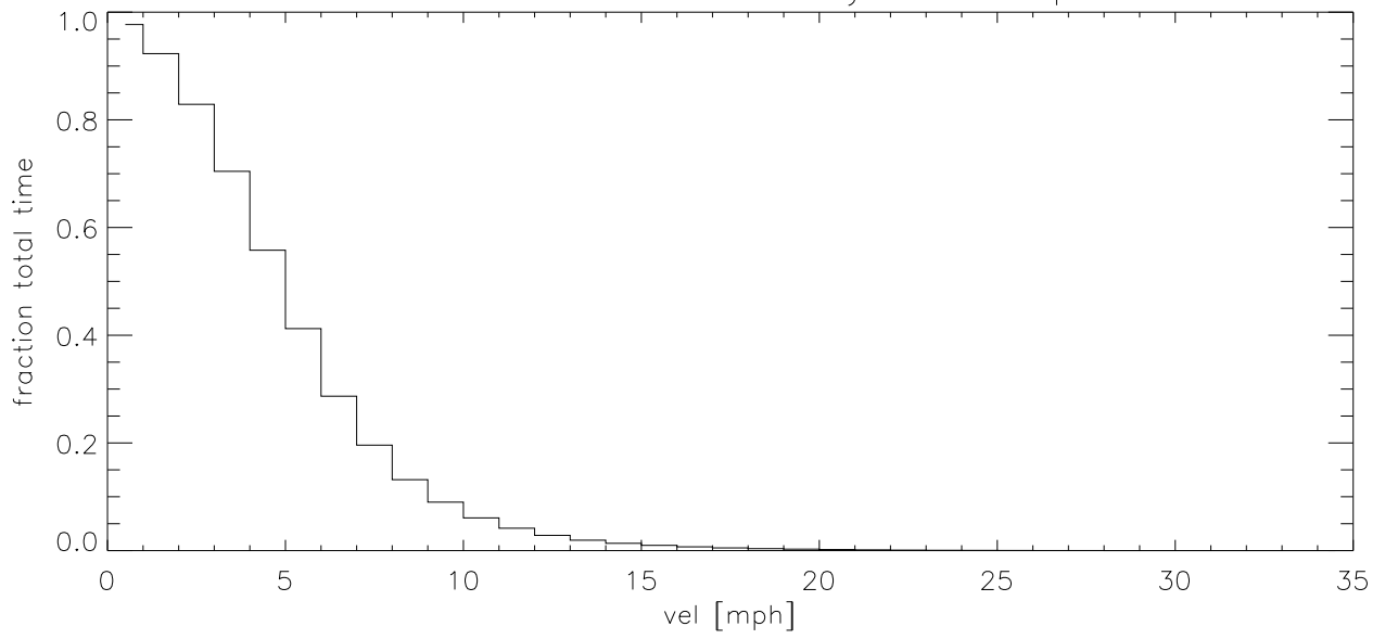
OCT07 Fraction of time wind velocity exceeds specified vel (blowup)
