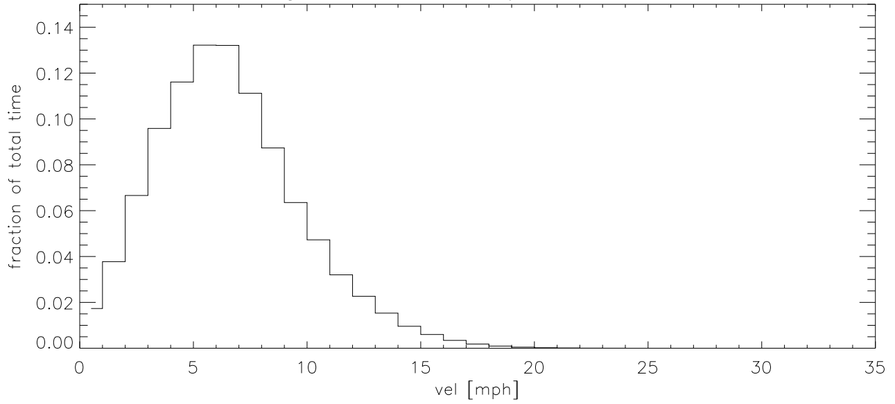
AUG06 Fraction of time wind velocity exceeds specified vel
