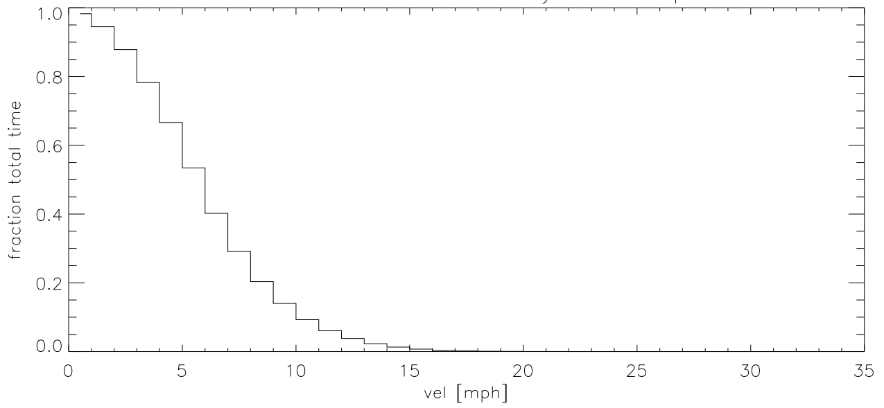
AUG06 Fraction of time wind velocity exceeds specified vel (blowup)
