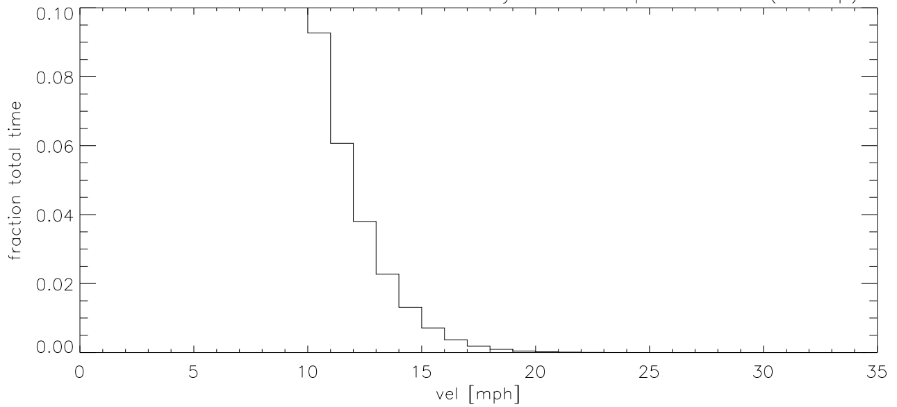
AUG06 Fraction of time wind velocity exceeds specified vel (blowup)
