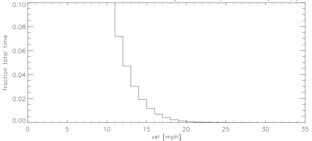
JUL06 Fraction of time wind velocity exceeds specified vel (blowup)
