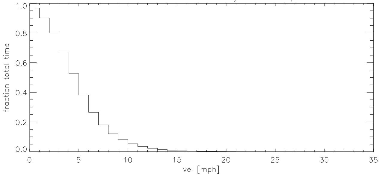
JUN06 Fraction of time wind velocity exceeds specified vel (blowup)
