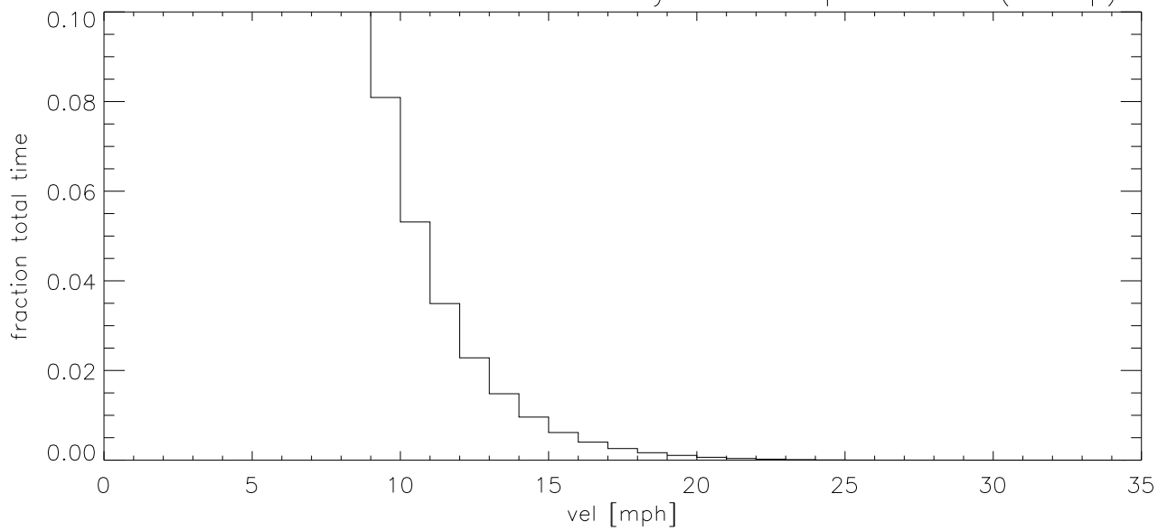
JUN06 Fraction of time wind velocity exceeds specified vel (blowup)
