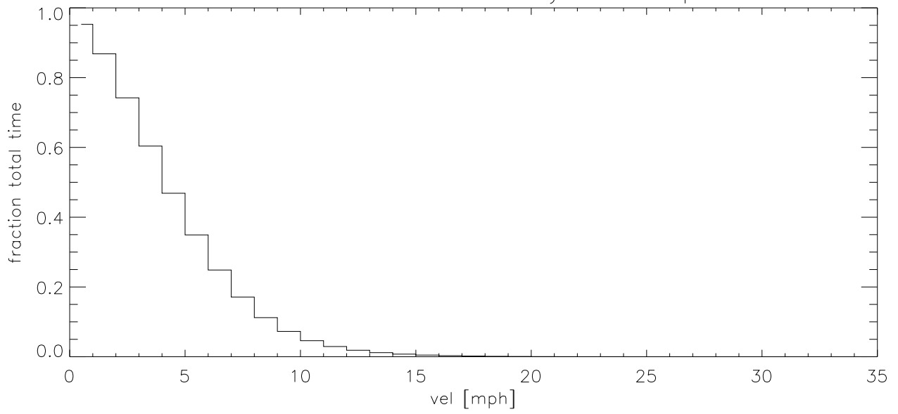
OCT05 Fraction of time wind velocity exceeds specified vel (blowup)
