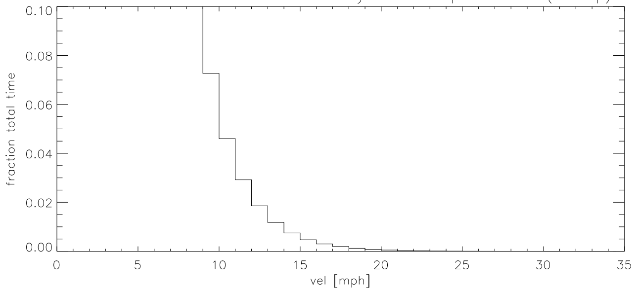
OCT05 Fraction of time wind velocity exceeds specified vel (blowup)
