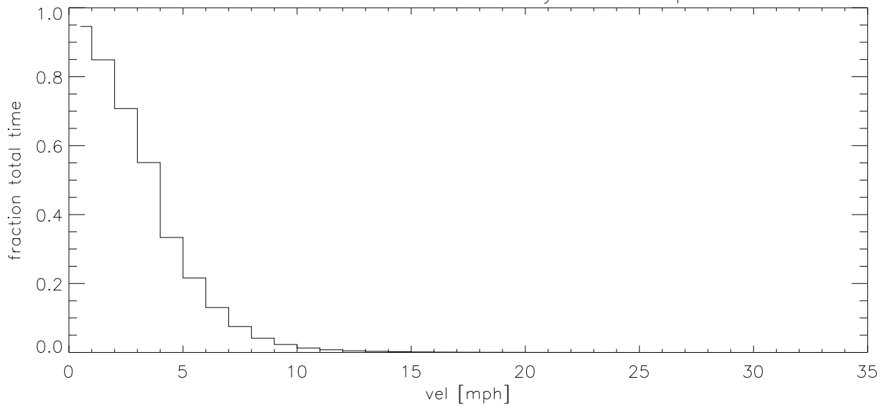
SEP05 Fraction of time wind velocity exceeds specified vel (blowup)
