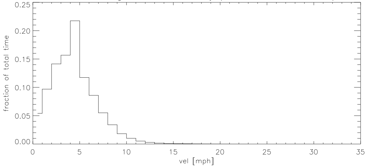
SEP05 Fraction of time wind velocity exceeds specified vel
