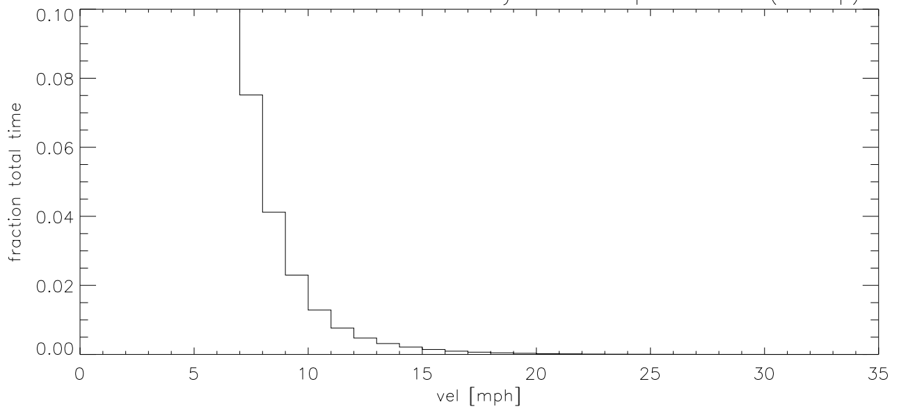
SEP05 Fraction of time wind velocity exceeds specified vel (blowup)
