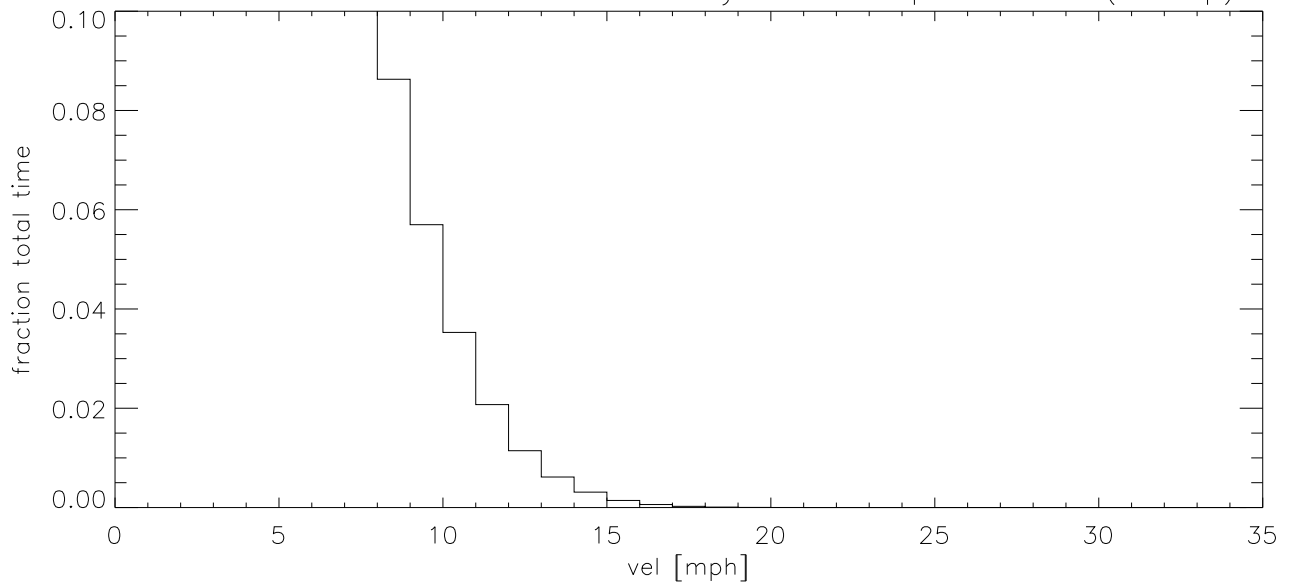
FEB05 Fraction of time wind velocity exceeds specified vel (blowup)
