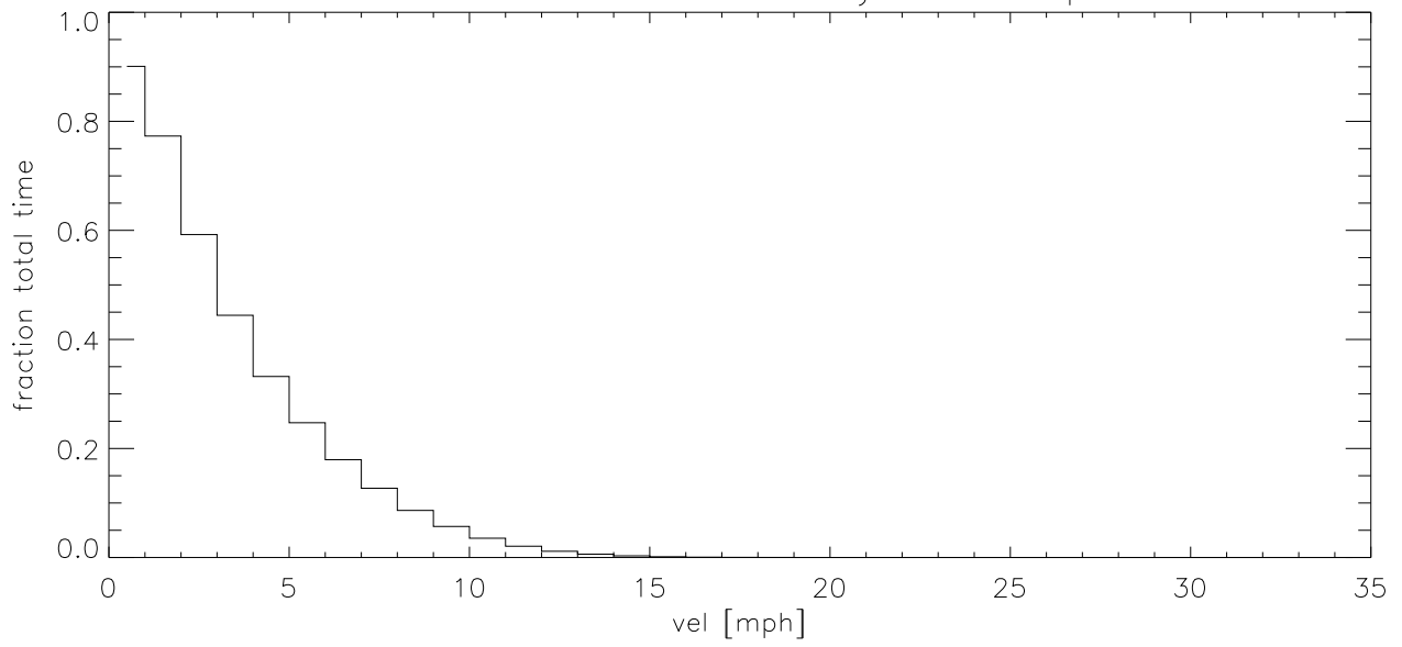
FEB05 Fraction of time wind velocity exceeds specified vel (blowup)
