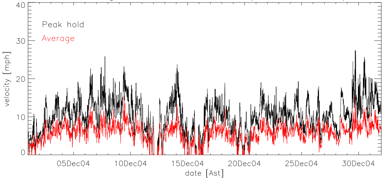
DEC04 Average, median velocity by hour of day
