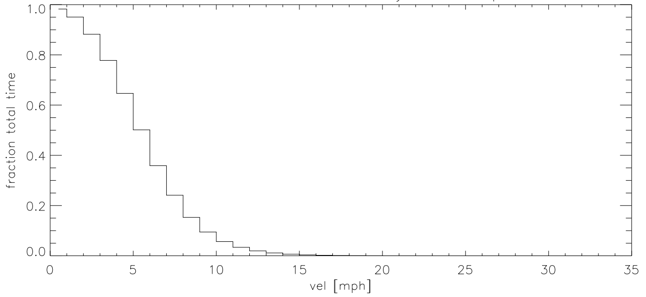
DEC04 Fraction of time wind velocity exceeds specified vel (blowup)
