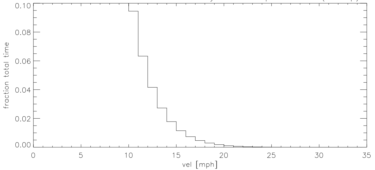
NOV04 Fraction of time wind velocity exceeds specified vel (blowup)
