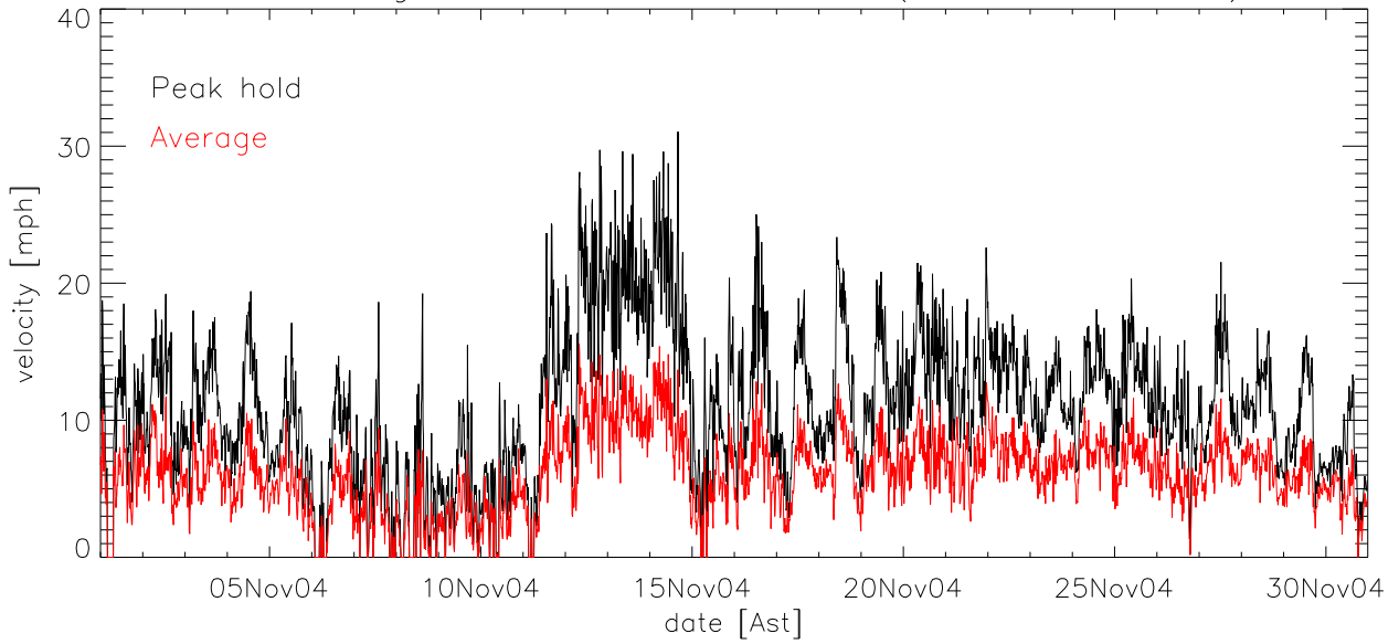
NOV04 Average, median velocity by hour of day
