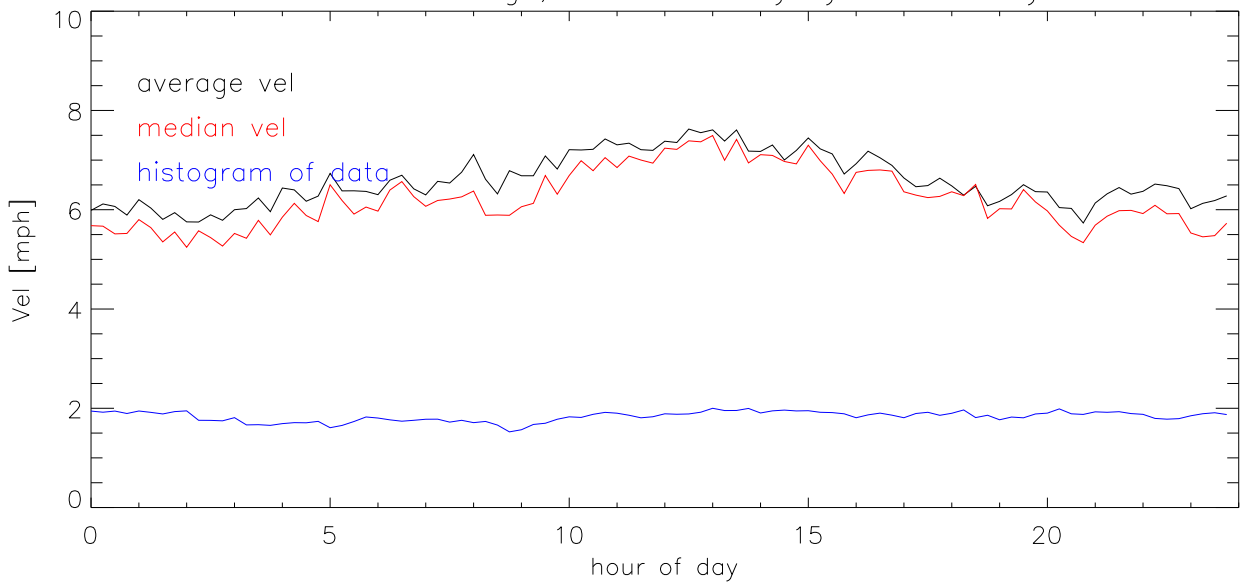
NOV04 Average, median velocity by direction
