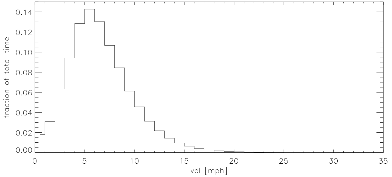
NOV04 Fraction of time wind velocity exceeds specified vel
