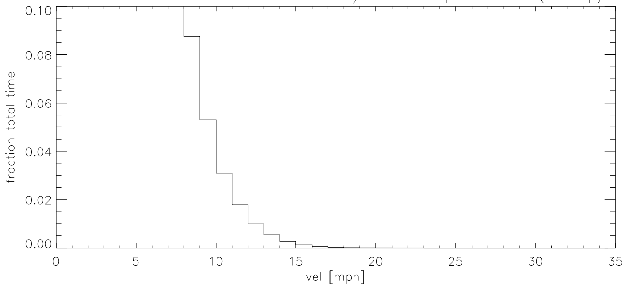
OCT04 Fraction of time wind velocity exceeds specified vel (blowup)
