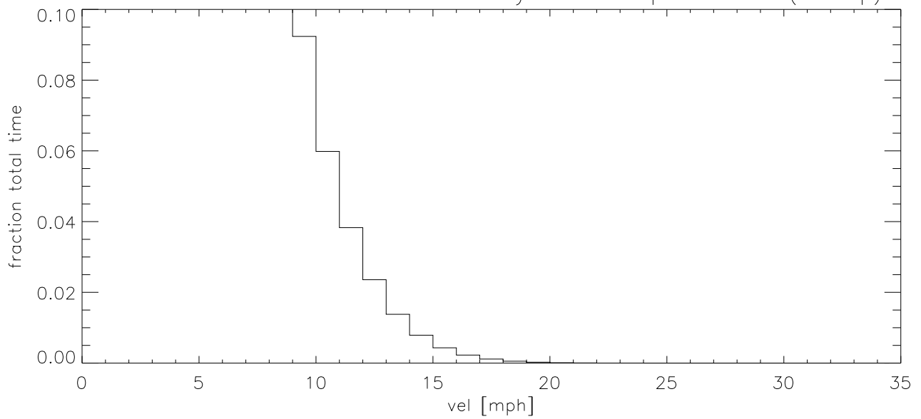
APR04 Fraction of time wind velocity exceeds specified vel (blowup)
