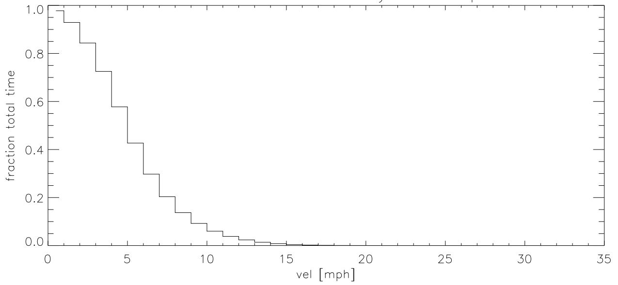
APR04 Fraction of time wind velocity exceeds specified vel (blowup)
