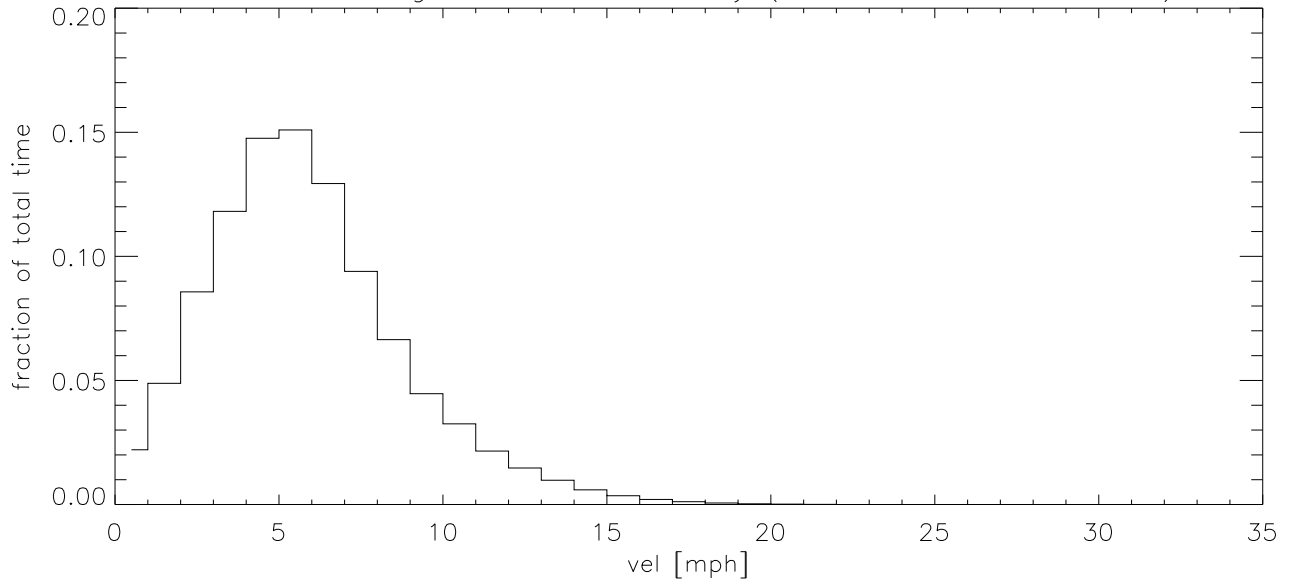
APR04 Fraction of time wind velocity exceeds specified vel
