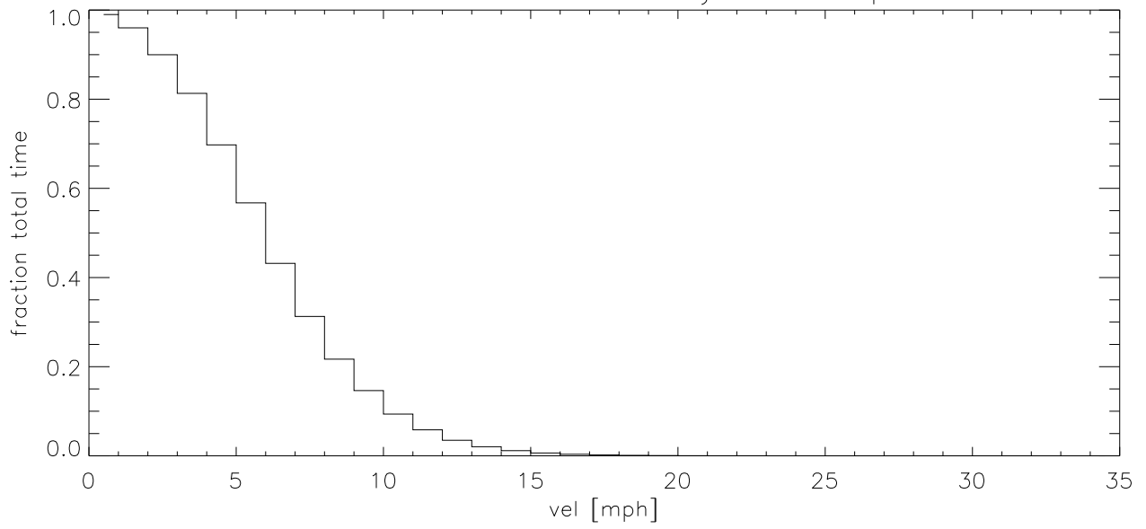
FEB04 Fraction of time wind velocity exceeds specified vel (blowup)
