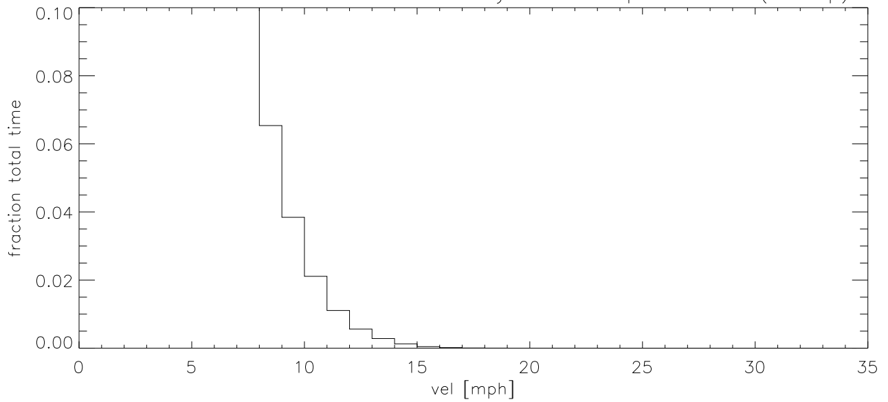
OCT03 Fraction of time wind velocity exceeds specified vel (blowup)
