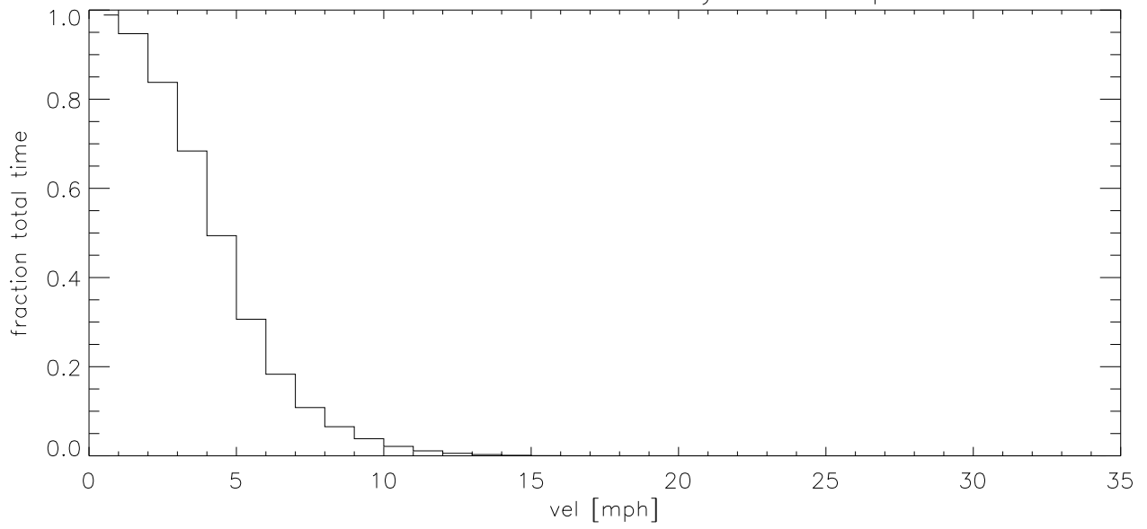
OCT03 Fraction of time wind velocity exceeds specified vel (blowup)
