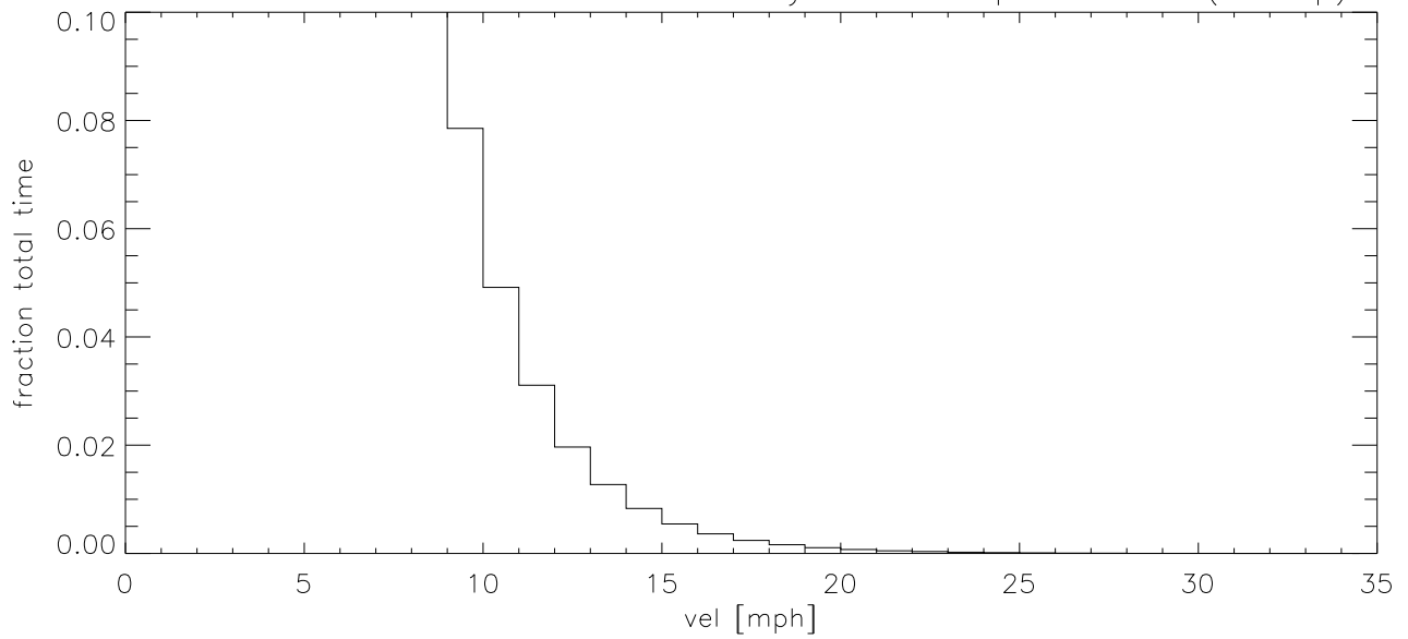
SEP03 Fraction of time wind velocity exceeds specified vel (blowup)
