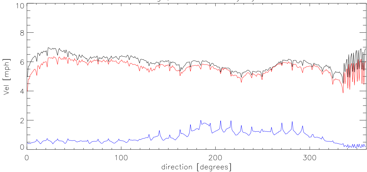
SEP03 Average, median velocity by direction
