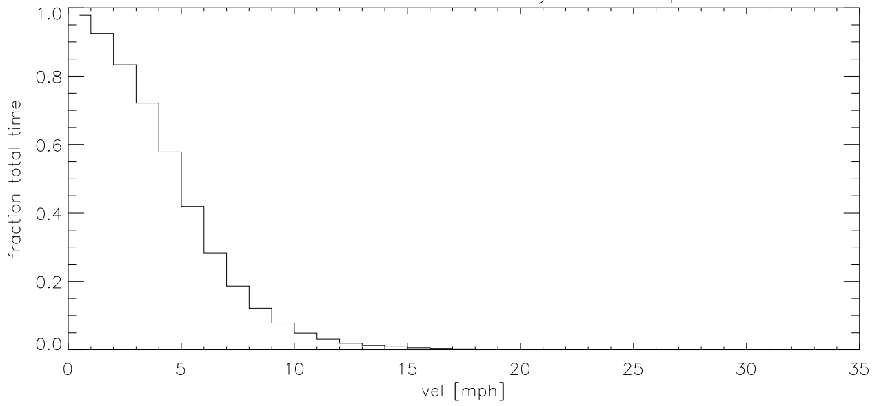
SEP03 Fraction of time wind velocity exceeds specified vel (blowup)
