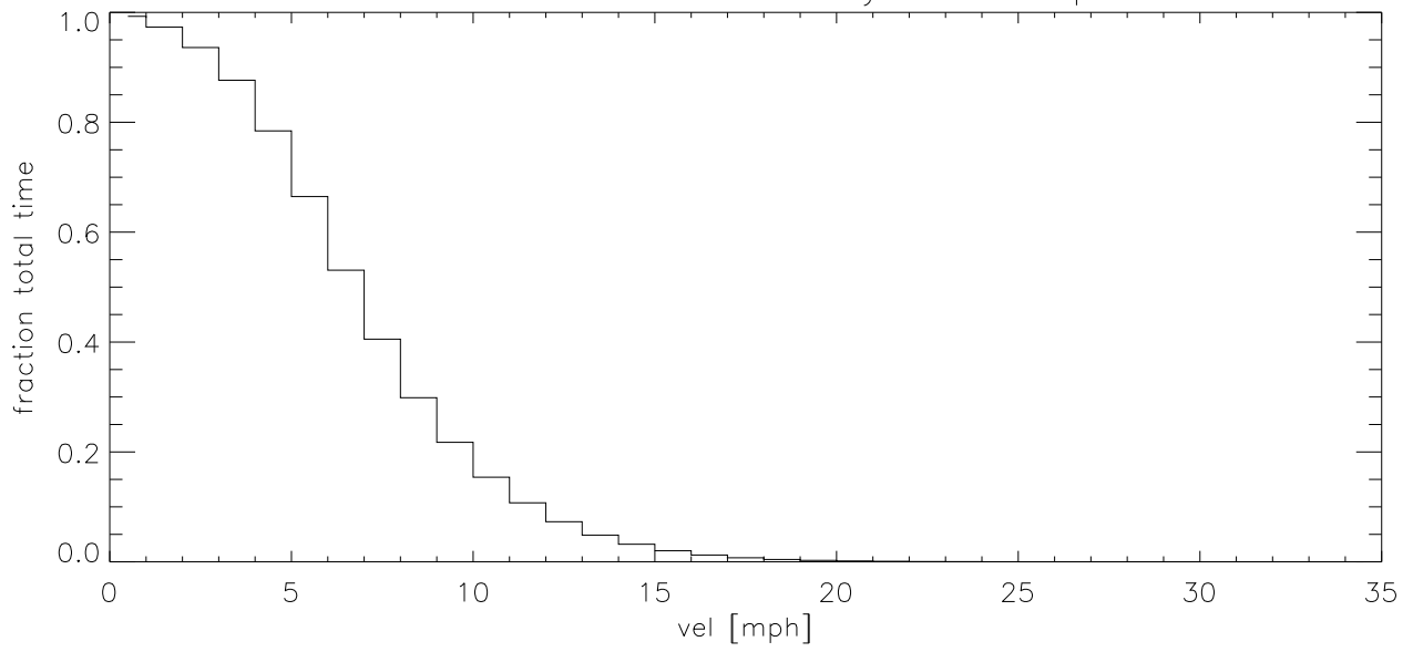
JUL03 Fraction of time wind velocity exceeds specified vel (blowup)
