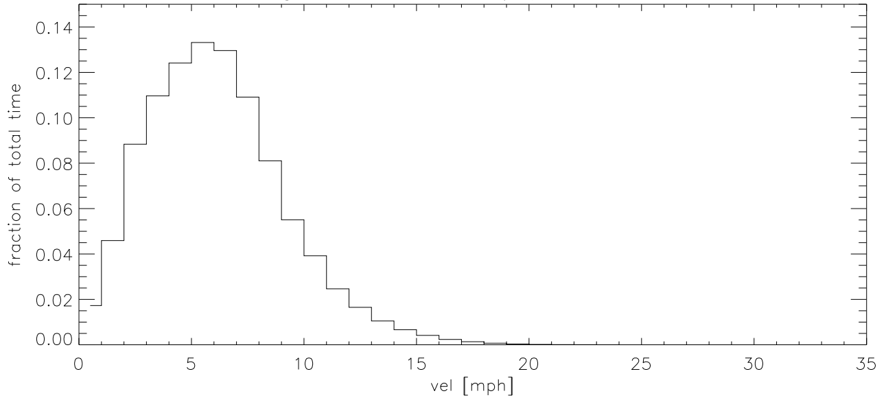
JUN03 Fraction of time wind velocity exceeds specified vel
