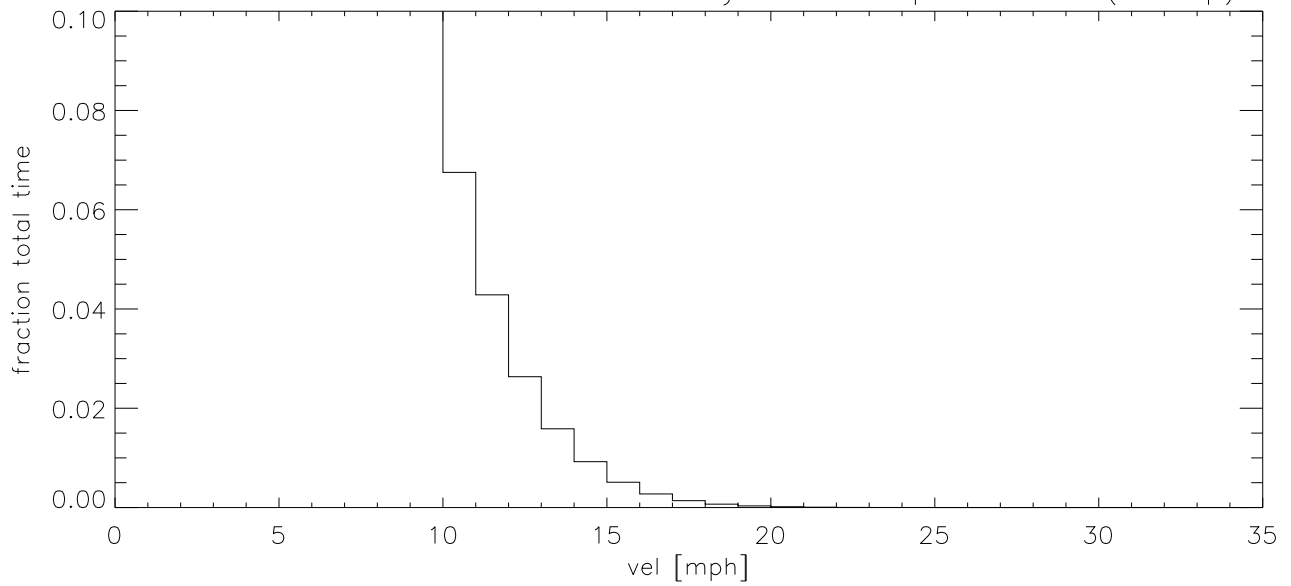
JUN03 Fraction of time wind velocity exceeds specified vel (blowup)
