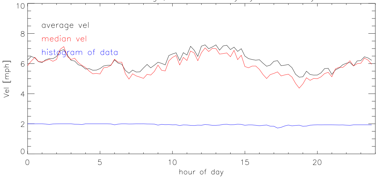
JUN03 Average, median velocity by direction
