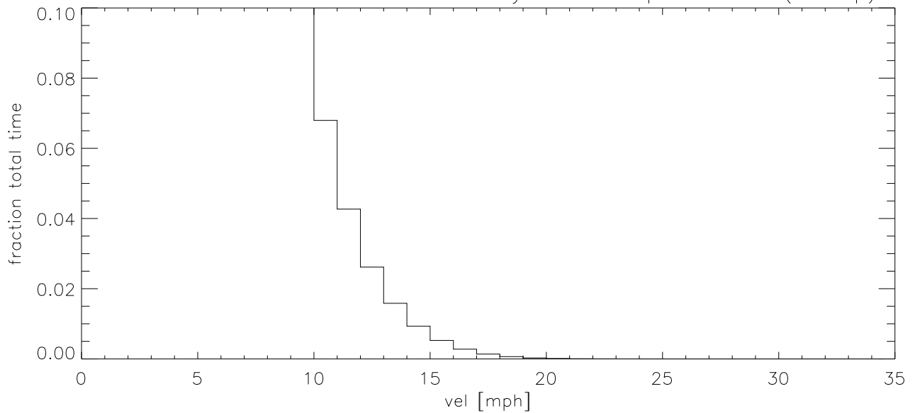
MAY03 Fraction of time wind velocity exceeds specified vel (blowup)
