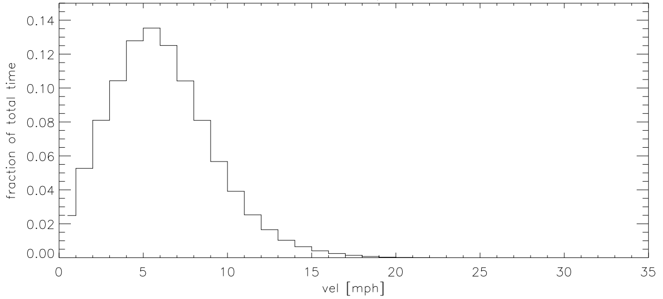
MAY03 Fraction of time wind velocity exceeds specified vel
