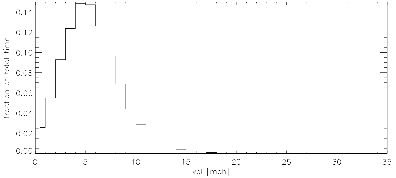
JAN03 Fraction of time wind velocity exceeds specified vel
