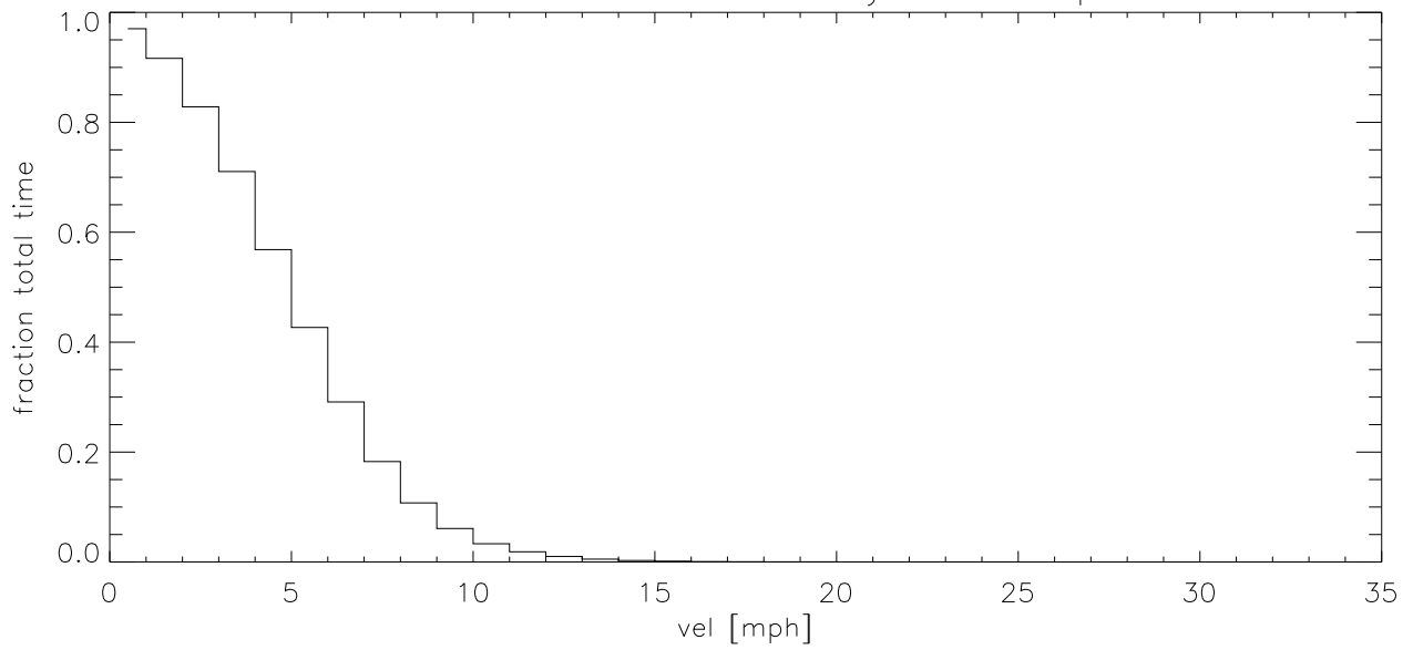
NOV02 Fraction of time wind velocity exceeds specified vel (blowup)
