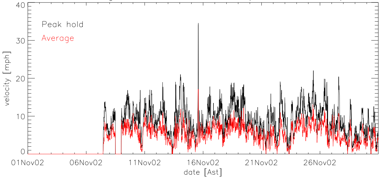
NOV02 Average, median velocity by hour of day
