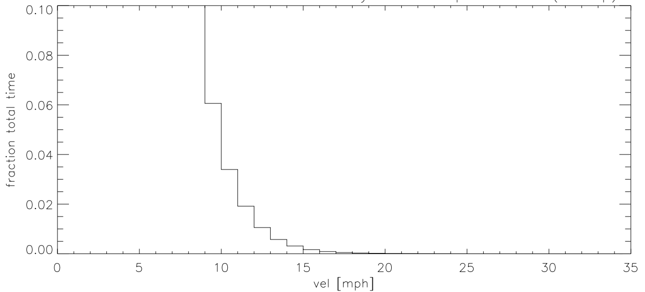
OCT02 Fraction of time wind velocity exceeds specified vel (blowup)
