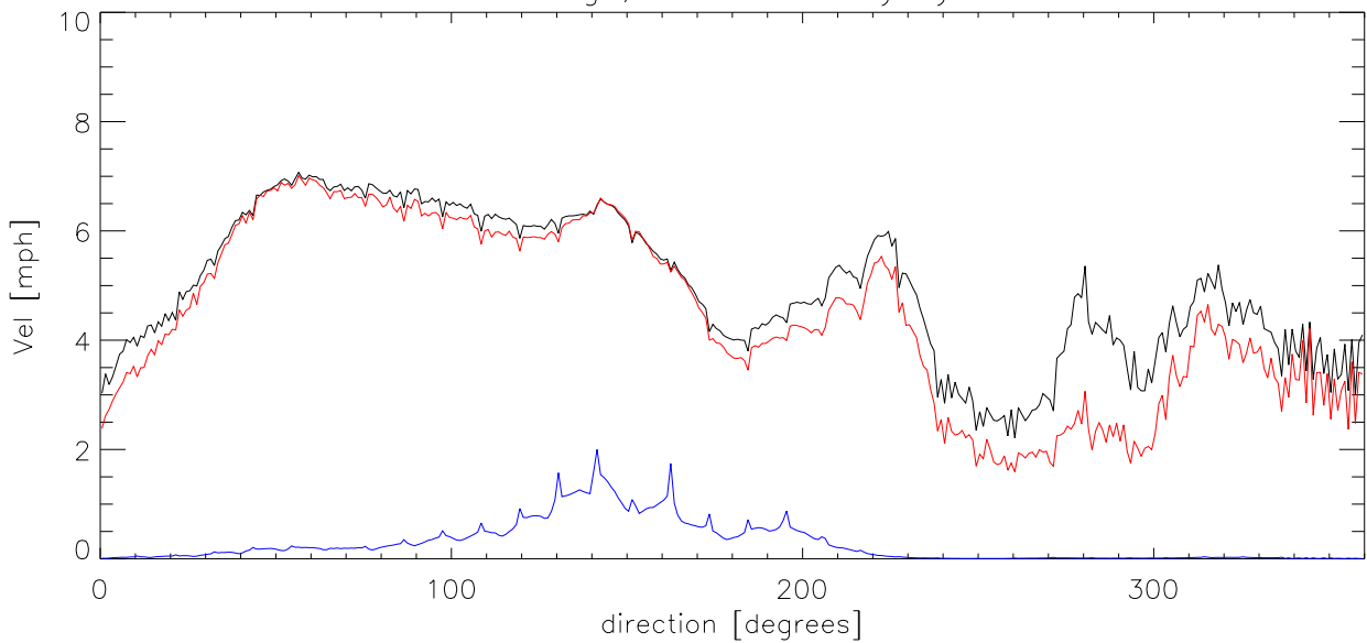
OCT02 Average, median velocity by direction
