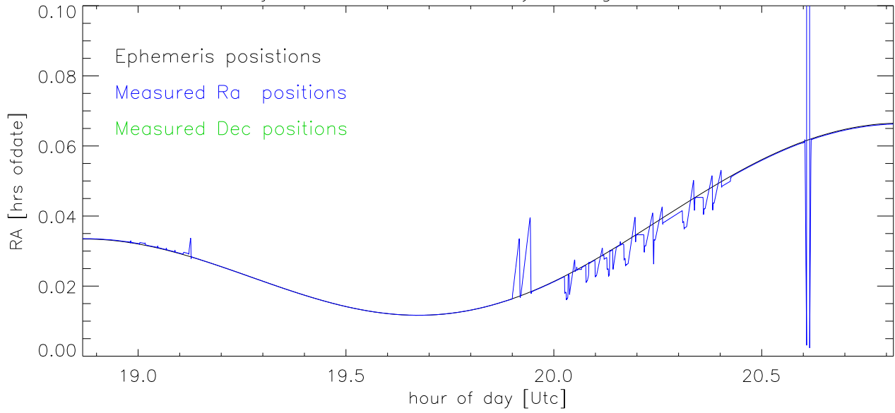
Dec vs hour of day during sband test
