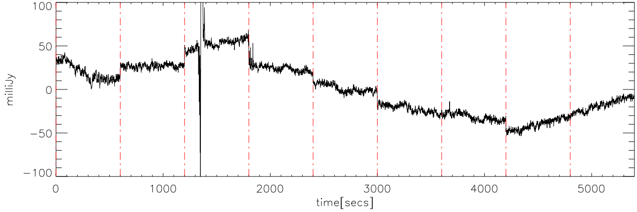
p2111 file:12 30dec08 (AST) StokesQ freq:4475.
