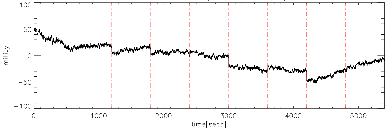
p2111 file:12 30dec08 (AST) StokesQ freq:4600.
