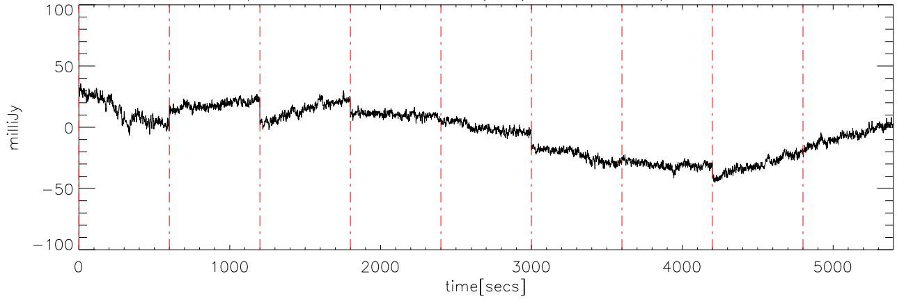
p2111 file:12 30dec08 (AST) StokesQ freq:4725.
